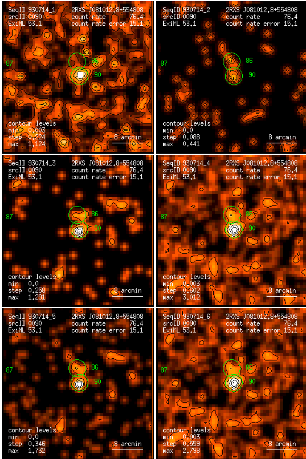
Figure 90: RASS 930714: detection 0090: band rate images, Gaussian filter: (1) PSPC channels 11 – 41, (2) 52 – 90, (3) 91 – 201, (4) 11 – 235, (5) 52 – 201, (6) 11 – 201. Broad band rates in counts/ks. Band rate contour levels in counts/ks/arcmin 2 .
