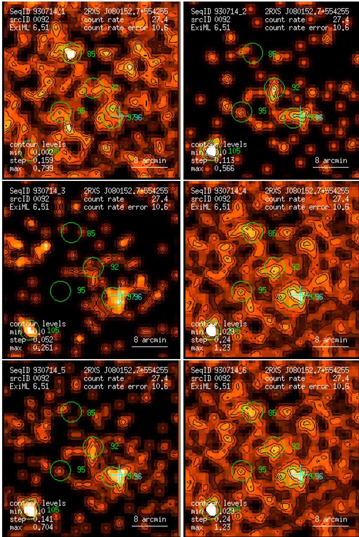
Figure 92: RASS 930714: detection 0092: band rate images, Gaussian filter: (1) PSPC channels 11 – 41, (2) 52 – 90, (3) 91 – 201, (4) 11 – 235, (5) 52 – 201, (6) 11 – 201. Broad band rates in counts/ks. Band rate contour levels in counts/ks/arcmin 2 .
