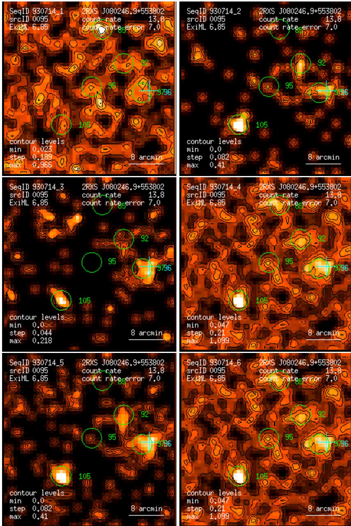
Figure 95: RASS 930714: detection 0095: band rate images, Gaussian filter: (1) PSPC channels 11 – 41, (2) 52 – 90, (3) 91 – 201, (4) 11 – 235, (5) 52 – 201, (6) 11 – 201. Broad band rates in counts/ks. Band rate contour levels in counts/ks/arcmin 2 .
