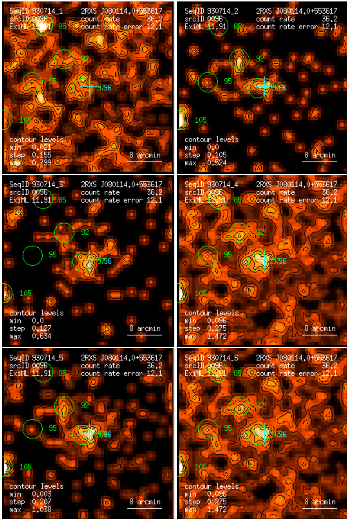
Figure 96: RASS 930714: detection 0096: band rate images, Gaussian filter: (1) PSPC channels 11 – 41, (2) 52 – 90, (3) 91 – 201, (4) 11 – 235, (5) 52 – 201, (6) 11 – 201. Broad band rates in counts/ks. Band rate contour levels in counts/ks/arcmin 2 .
