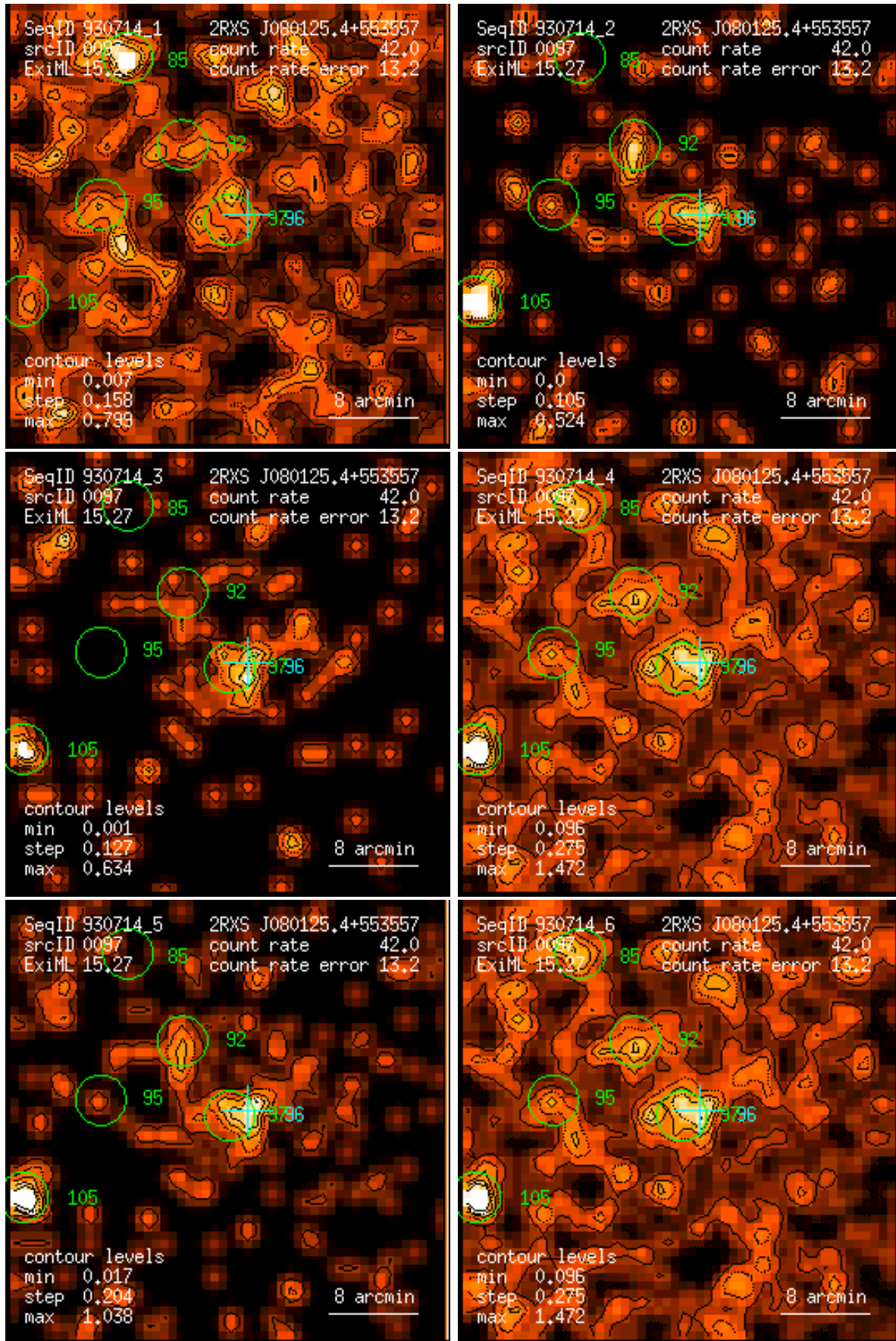
Figure 97: RASS 930714: detection 0097: band rate images, Gaussian filter: (1) PSPC channels 11 – 41, (2) 52 – 90, (3) 91 – 201, (4) 11 – 235, (5) 52 – 201, (6) 11 – 201. Broad band rates in counts/ks. Band rate contour levels in counts/ks/arcmin 2 .
