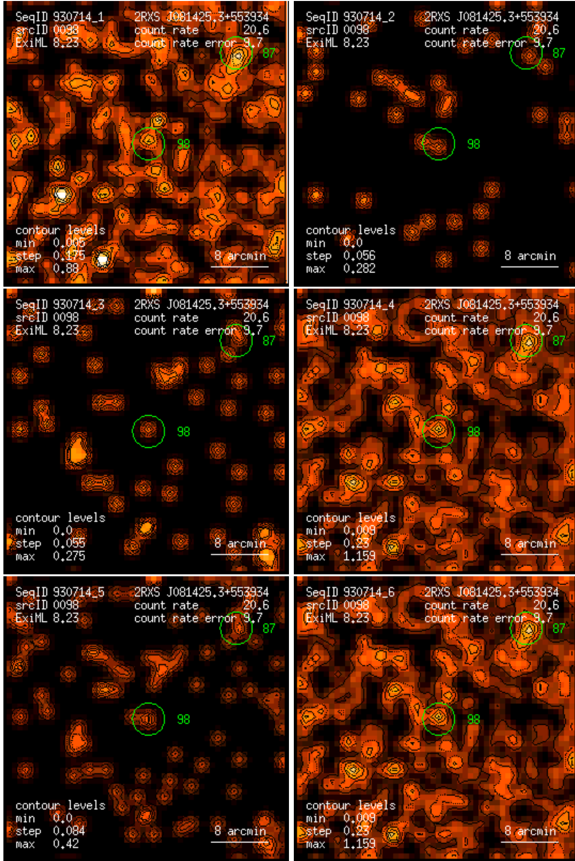
Figure 98: RASS 930714: detection 0098: band rate images, Gaussian filter: (1) PSPC channels 11 – 41, (2) 52 – 90, (3) 91 – 201, (4) 11 – 235, (5) 52 – 201, (6) 11 – 201. Broad band rates in counts/ks. Band rate contour levels in counts/ks/arcmin 2 .
