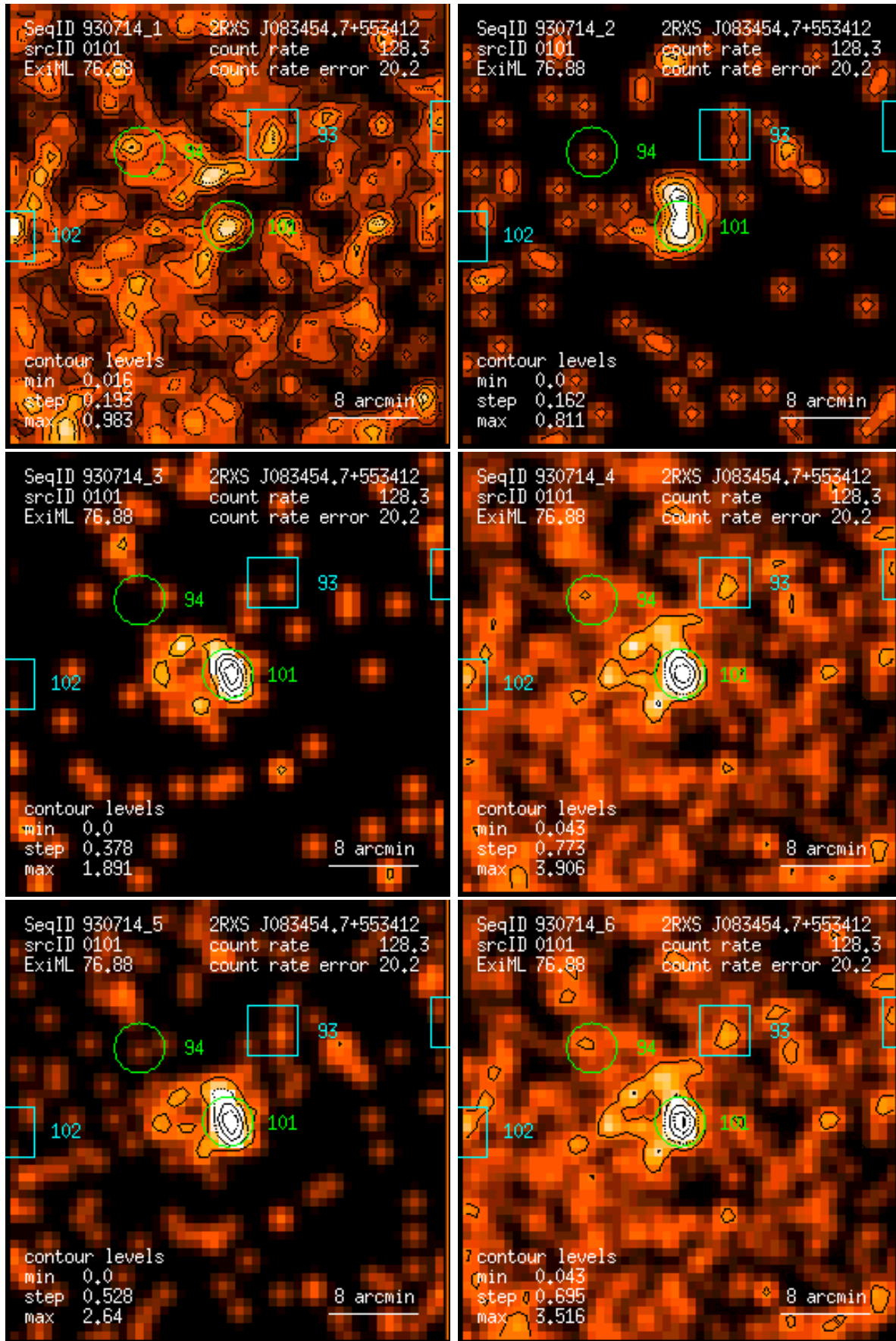
Figure 101: RASS 930714: detection 0101: band rate images, Gaussian filter: (1) PSPC channels 11 – 41, (2) 52 – 90, (3) 91 – 201, (4) 11 – 235, (5) 52 – 201, (6) 11 – 201. Broad band rates in counts/ks. Band rate contour levels in counts/ks/arcmin 2 .
