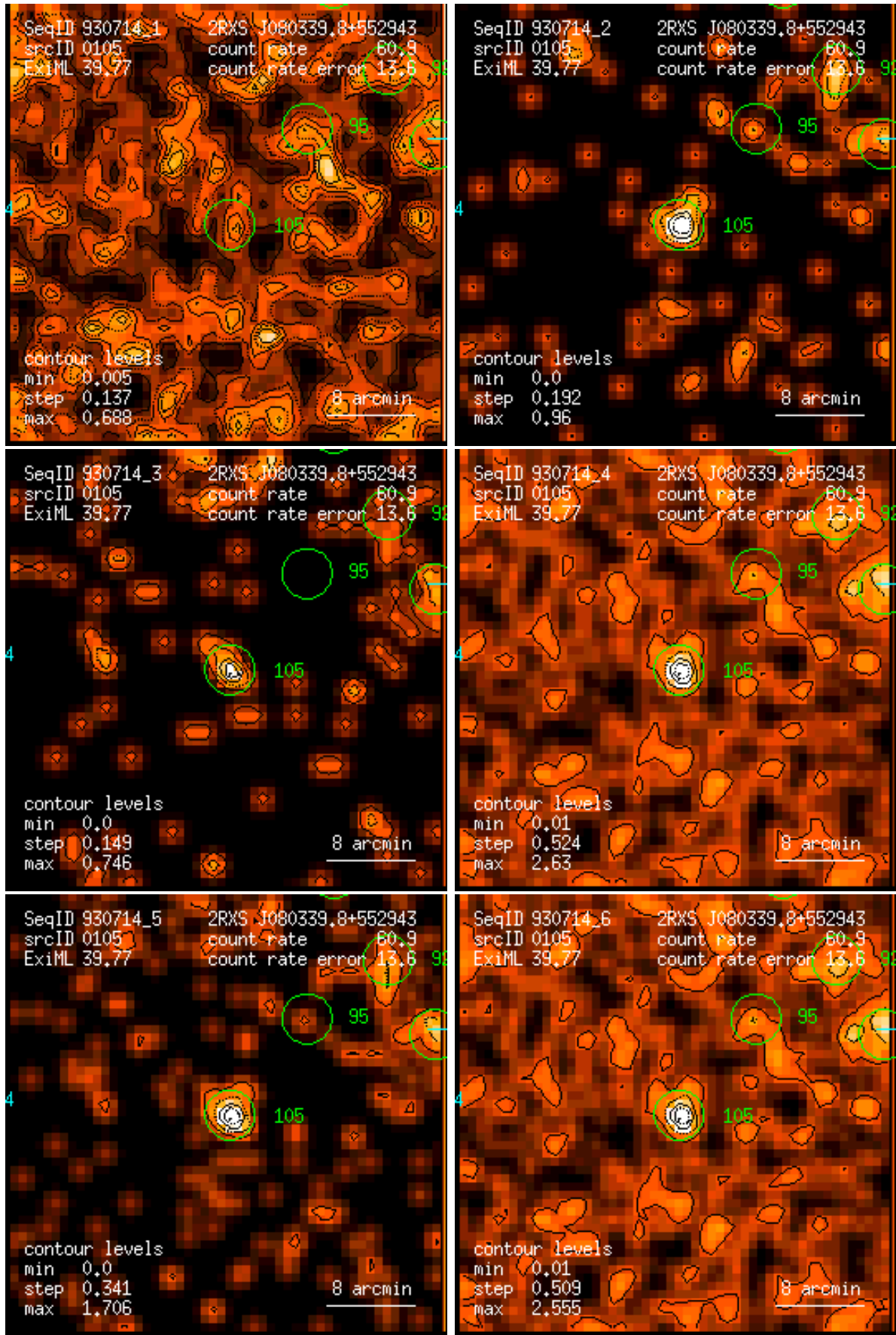
Figure 105: RASS 930714: detection 0105: band rate images, Gaussian filter: (1) PSPC channels 11 – 41, (2) 52 – 90, (3) 91 – 201, (4) 11 – 235, (5) 52 – 201, (6) 11 – 201. Broad band rates in counts/ks. Band rate contour levels in counts/ks/arcmin 2 .
