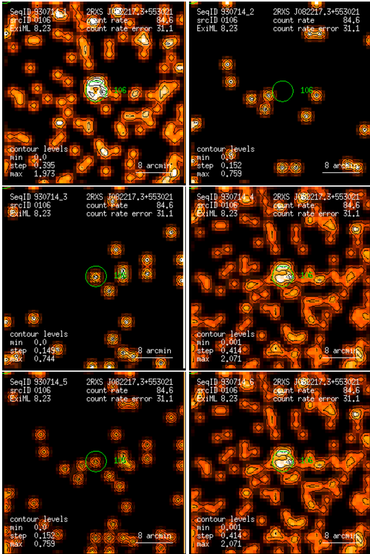
Figure 106: RASS 930714: detection 0106: band rate images, Gaussian filter: (1) PSPC channels 11 – 41, (2) 52 – 90, (3) 91 – 201, (4) 11 – 235, (5) 52 – 201, (6) 11 – 201. Broad band rates in counts/ks. Band rate contour levels in counts/ks/arcmin 2 .
