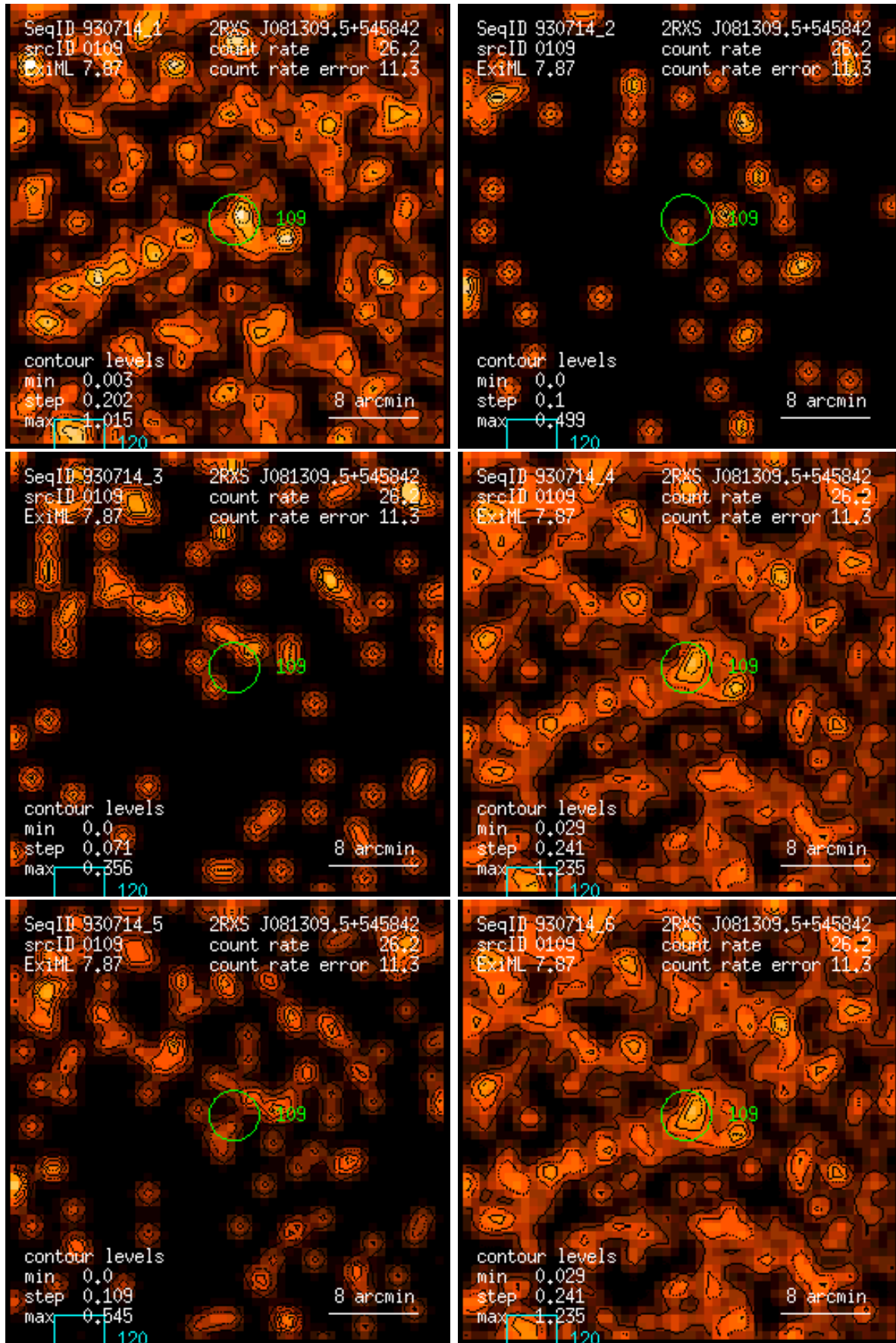
Figure 109: RASS 930714: detection 0109: band rate images, Gaussian filter: (1) PSPC channels 11 – 41, (2) 52 – 90, (3) 91 – 201, (4) 11 – 235, (5) 52 – 201, (6) 11 – 201. Broad band rates in counts/ks. Band rate contour levels in counts/ks/arcmin 2 .
