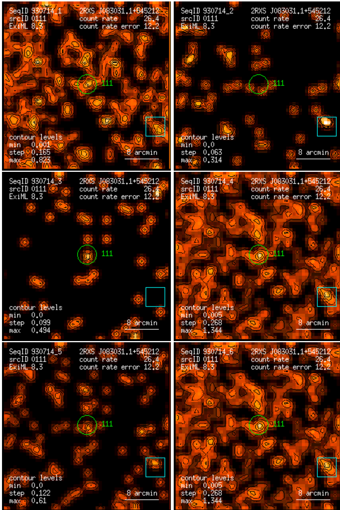
Figure 111: RASS 930714: detection 0111: band rate images, Gaussian filter: (1) PSPC channels 11 – 41, (2) 52 – 90, (3) 91 – 201, (4) 11 – 235, (5) 52 – 201, (6) 11 – 201. Broad band rates in counts/ks. Band rate contour levels in counts/ks/arcmin 2 .
