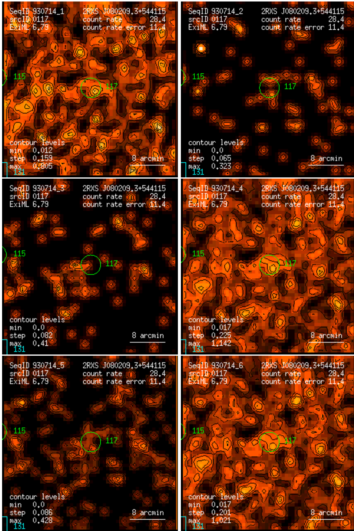
Figure 117: RASS 930714: detection 0117: band rate images, Gaussian filter: (1) PSPC channels 11 – 41, (2) 52 – 90, (3) 91 – 201, (4) 11 – 235, (5) 52 – 201, (6) 11 – 201. Broad band rates in counts/ks. Band rate contour levels in counts/ks/arcmin 2 .
