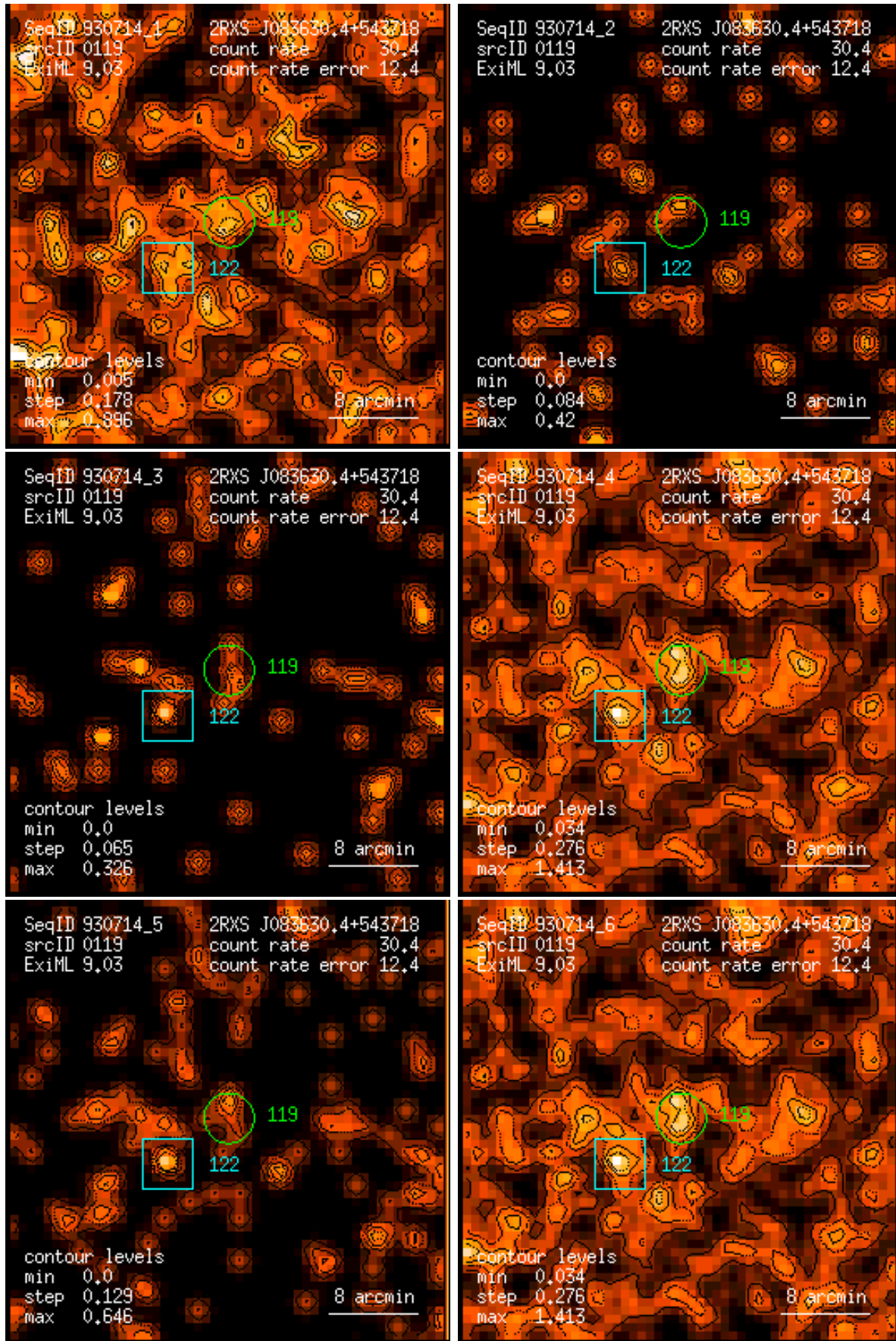
Figure 119: RASS 930714: detection 0119: band rate images, Gaussian filter: (1) PSPC channels 11 – 41, (2) 52 – 90, (3) 91 – 201, (4) 11 – 235, (5) 52 – 201, (6) 11 – 201. Broad band rates in counts/ks. Band rate contour levels in counts/ks/arcmin 2 .
