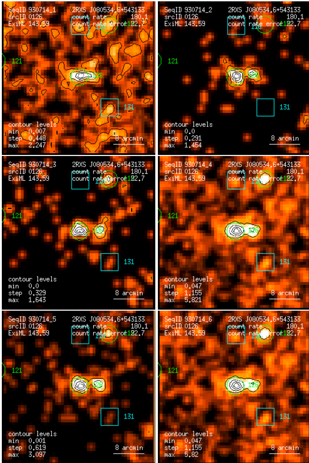
Figure 126: RASS 930714: detection 0126: band rate images, Gaussian filter: (1) PSPC channels 11 – 41, (2) 52 – 90, (3) 91 – 201, (4) 11 – 235, (5) 52 – 201, (6) 11 – 201. Broad band rates in counts/ks. Band rate contour levels in counts/ks/arcmin 2 .
