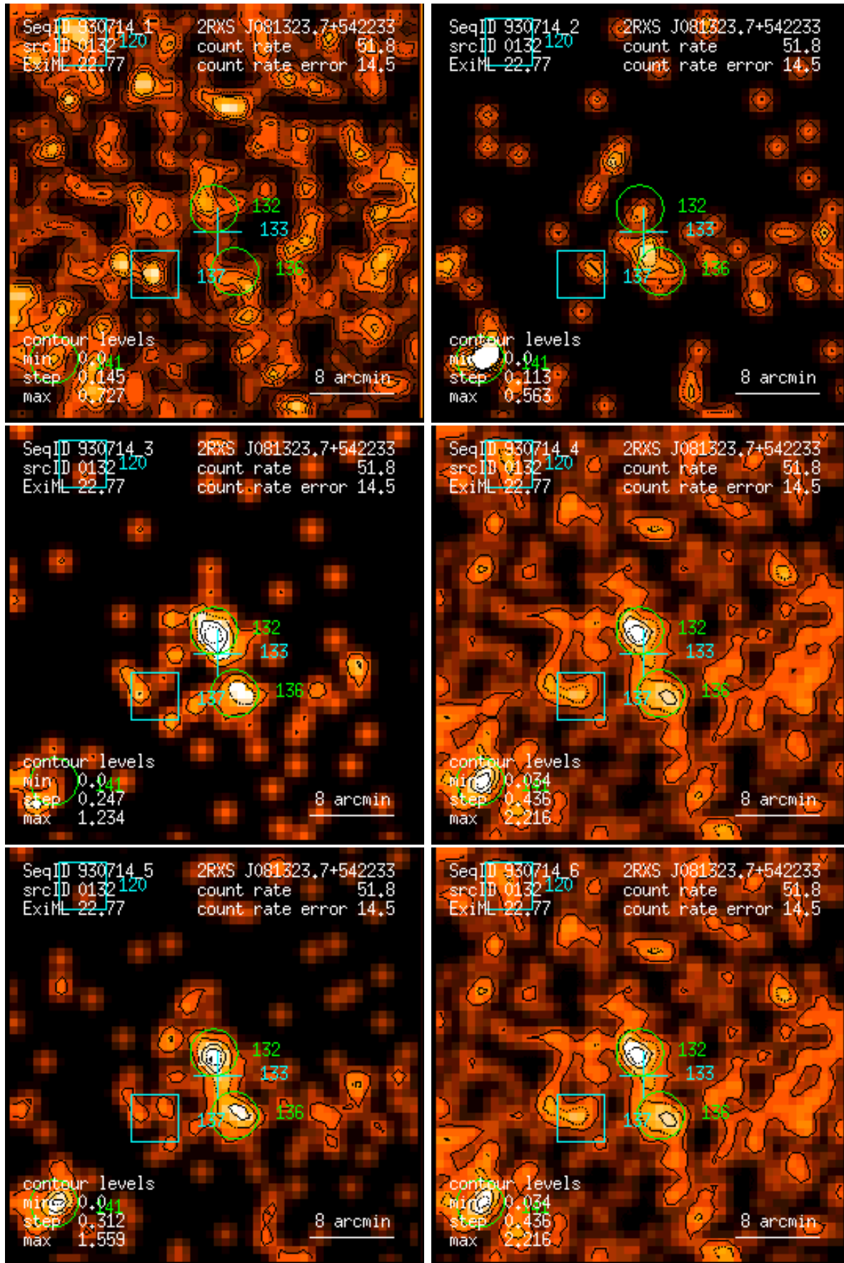
Figure 132: RASS 930714: detection 0132: band rate images, Gaussian filter: (1) PSPC channels 11 – 41, (2) 52 – 90, (3) 91 – 201, (4) 11 – 235, (5) 52 – 201, (6) 11 – 201. Broad band rates in counts/ks. Band rate contour levels in counts/ks/arcmin 2 .
