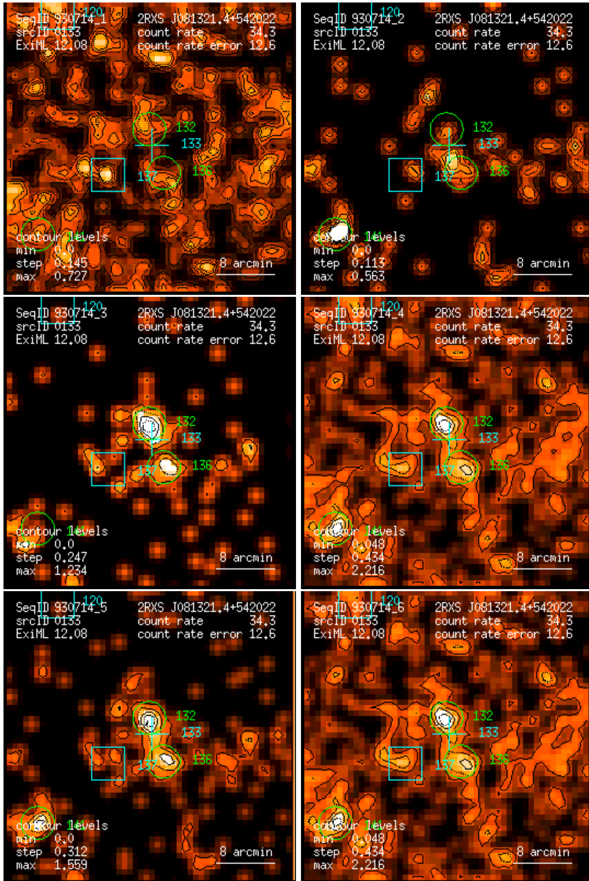
Figure 133: RASS 930714: detection 0133: band rate images, Gaussian filter: (1) PSPC channels 11 – 41, (2) 52 – 90, (3) 91 – 201, (4) 11 – 235, (5) 52 – 201, (6) 11 – 201. Broad band rates in counts/ks. Band rate contour levels in counts/ks/arcmin 2 .
