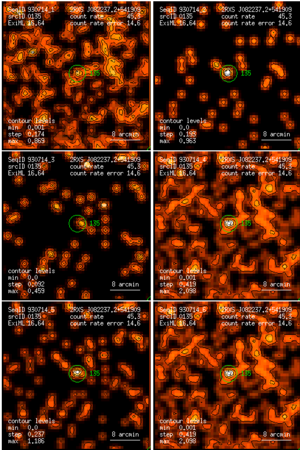
Figure 135: RASS 930714: detection 0135: band rate images, Gaussian filter: (1) PSPC channels 11 – 41, (2) 52 – 90, (3) 91 – 201, (4) 11 – 235, (5) 52 – 201, (6) 11 – 201. Broad band rates in counts/ks. Band rate contour levels in counts/ks/arcmin 2 .
