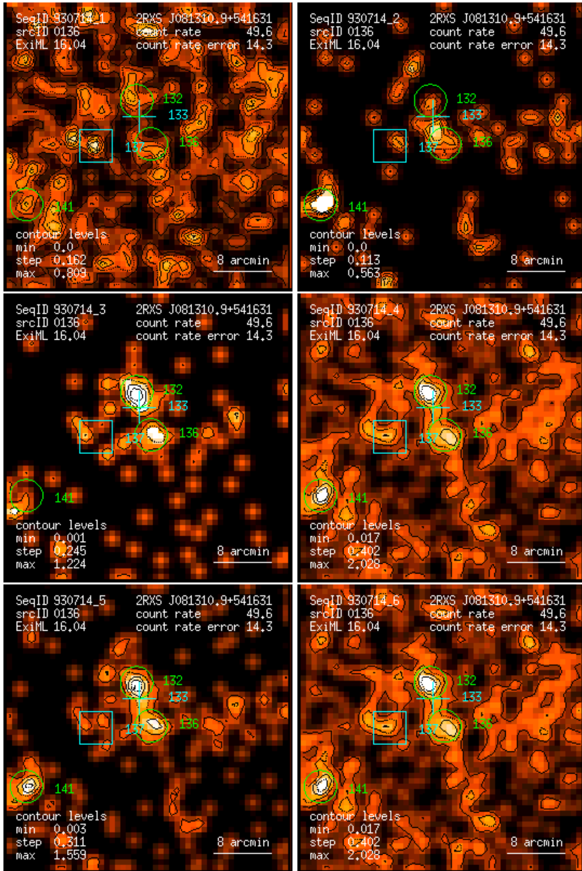
Figure 136: RASS 930714: detection 0136: band rate images, Gaussian filter: (1) PSPC channels 11 – 41, (2) 52 – 90, (3) 91 – 201, (4) 11 – 235, (5) 52 – 201, (6) 11 – 201. Broad band rates in counts/ks. Band rate contour levels in counts/ks/arcmin 2 .
