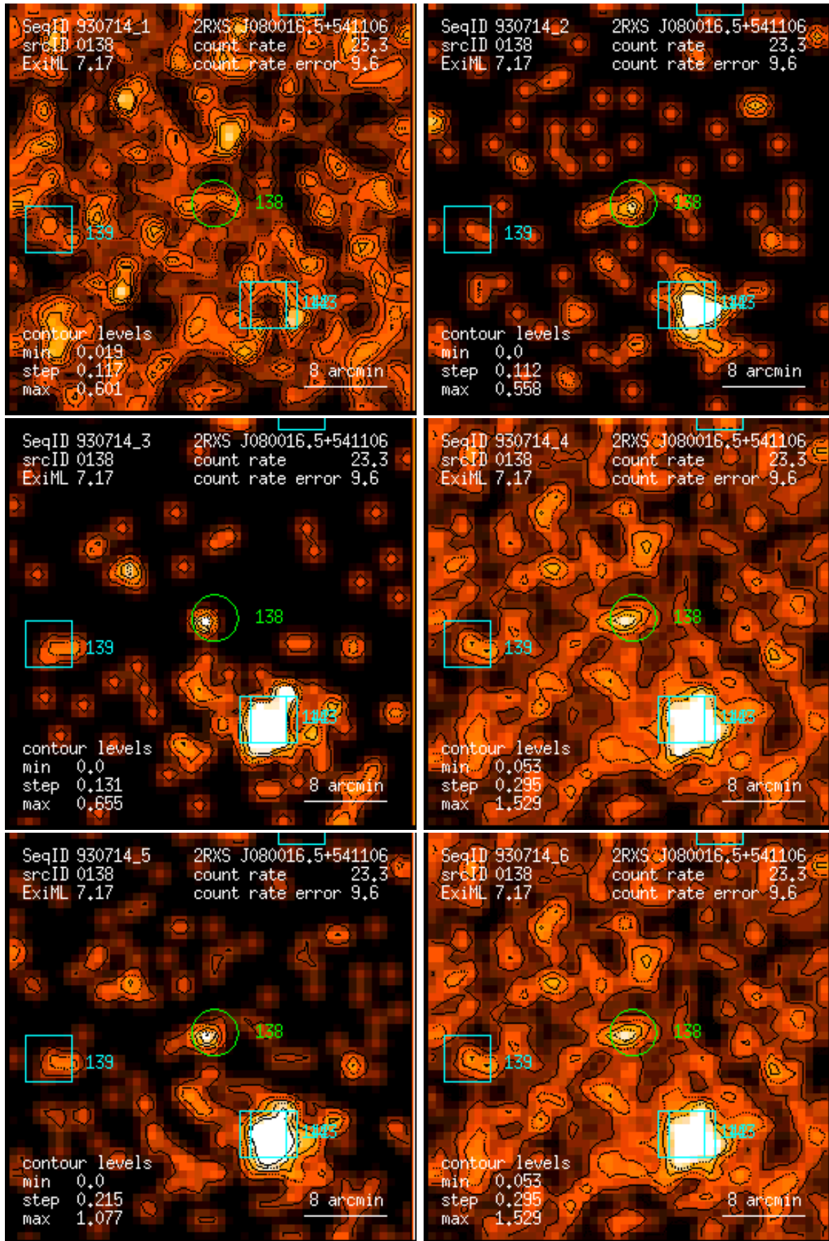
Figure 138: RASS 930714: detection 0138: band rate images, Gaussian filter: (1) PSPC channels 11 – 41, (2) 52 – 90, (3) 91 – 201, (4) 11 – 235, (5) 52 – 201, (6) 11 – 201. Broad band rates in counts/ks. Band rate contour levels in counts/ks/arcmin 2 .
