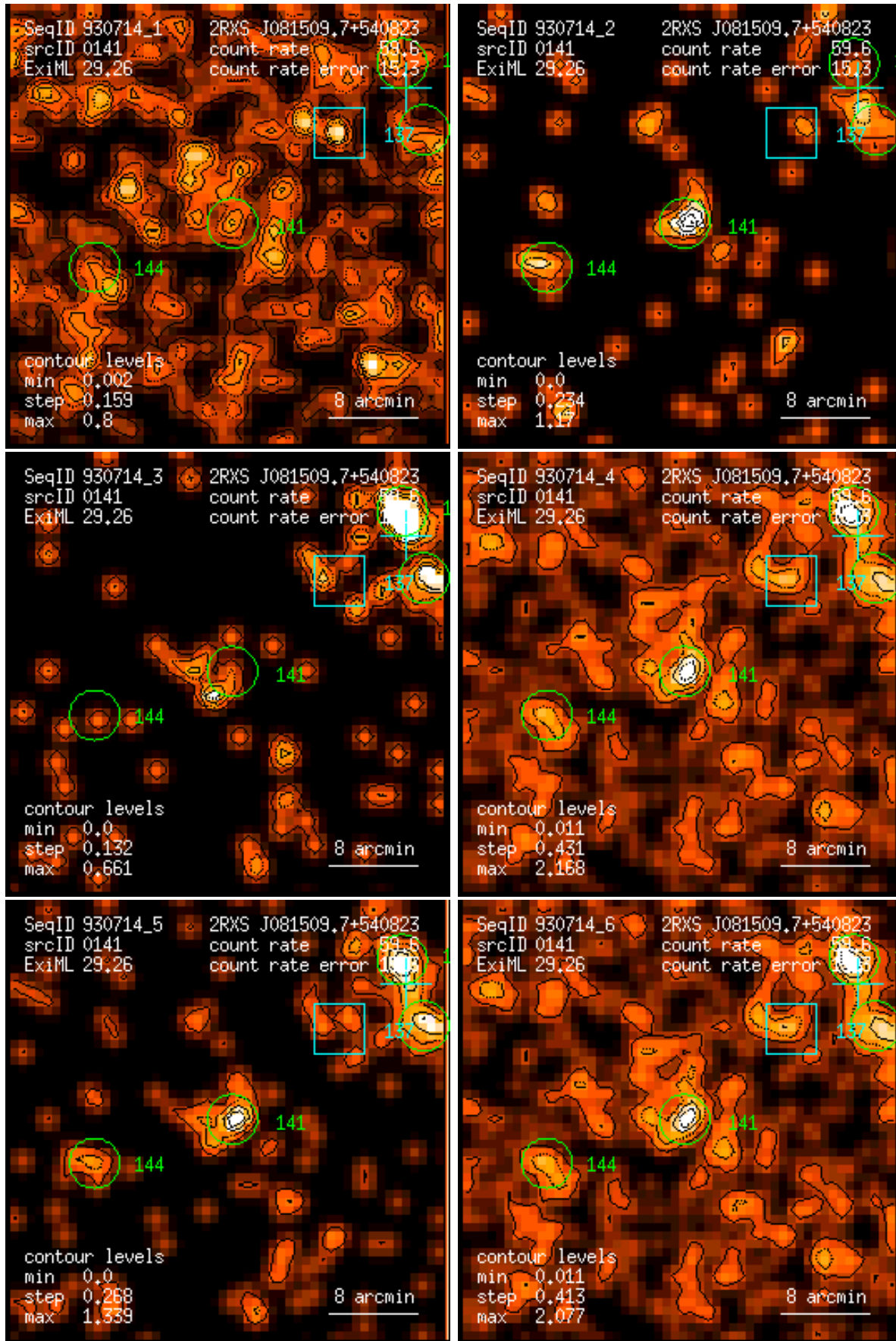
Figure 141: RASS 930714: detection 0141: band rate images, Gaussian filter: (1) PSPC channels 11 – 41, (2) 52 – 90, (3) 91 – 201, (4) 11 – 235, (5) 52 – 201, (6) 11 – 201. Broad band rates in counts/ks. Band rate contour levels in counts/ks/arcmin 2 .
