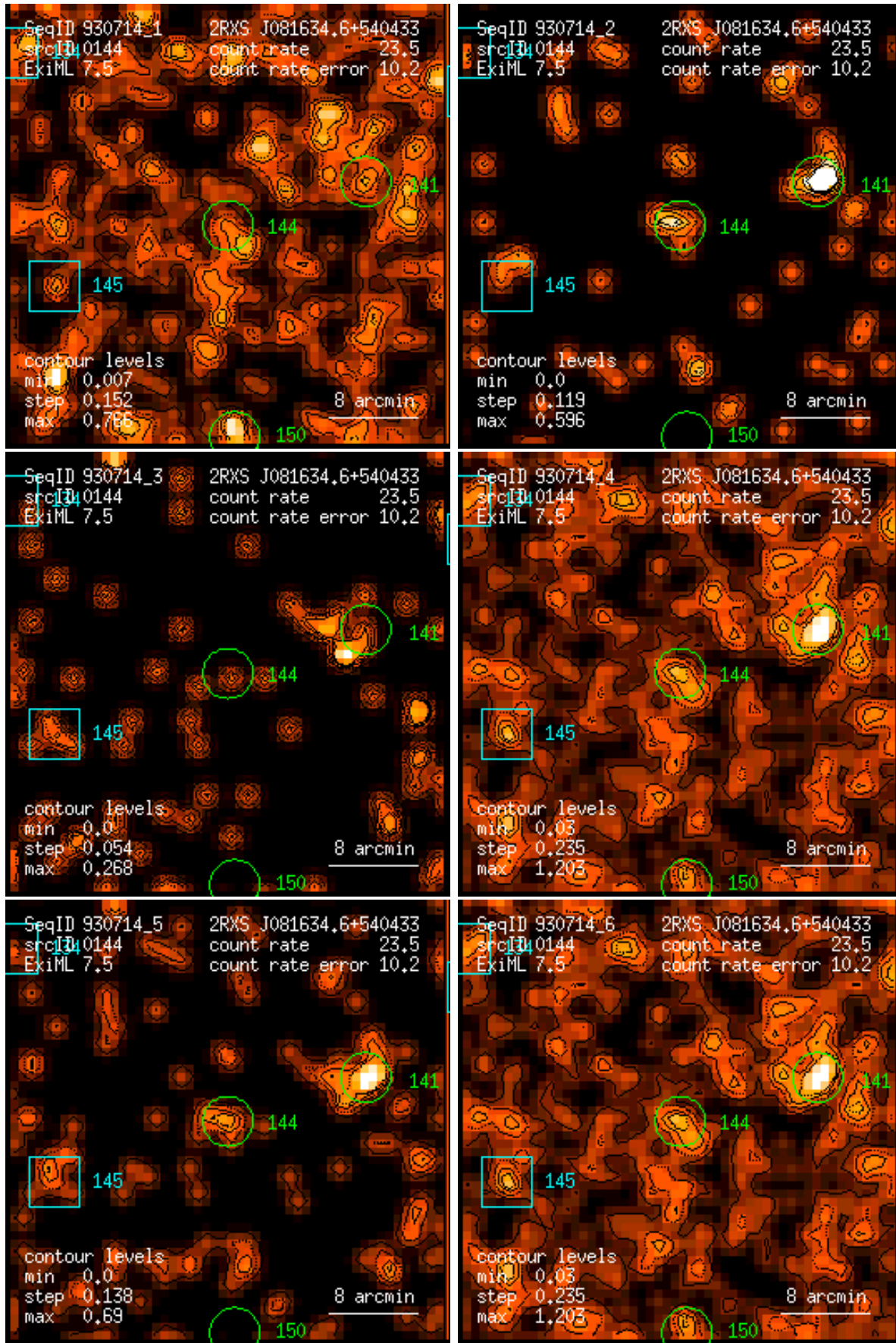
Figure 144: RASS 930714: detection 0144: band rate images, Gaussian filter: (1) PSPC channels 11 – 41, (2) 52 – 90, (3) 91 – 201, (4) 11 – 235, (5) 52 – 201, (6) 11 – 201. Broad band rates in counts/ks. Band rate contour levels in counts/ks/arcmin 2 .
