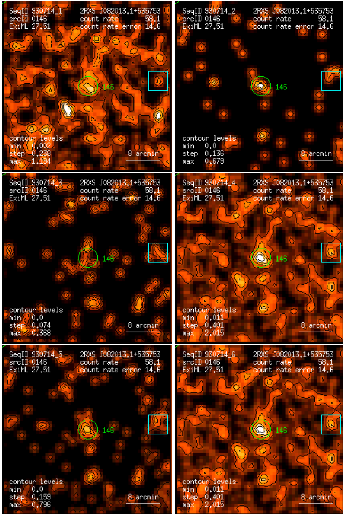
Figure 146: RASS 930714: detection 0146: band rate images, Gaussian filter: (1) PSPC channels 11 – 41, (2) 52 – 90, (3) 91 – 201, (4) 11 – 235, (5) 52 – 201, (6) 11 – 201. Broad band rates in counts/ks. Band rate contour levels in counts/ks/arcmin 2 .
