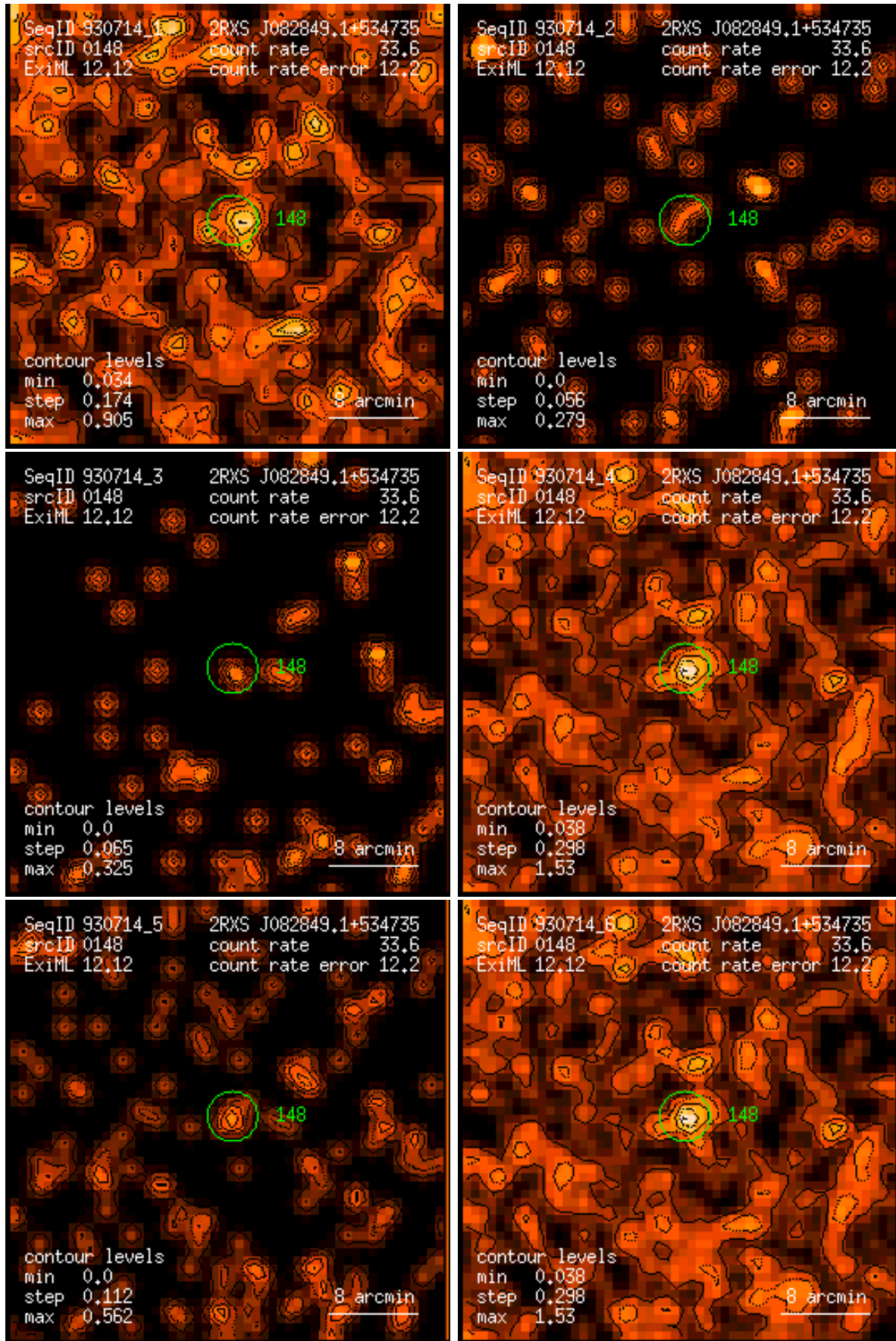
Figure 148: RASS 930714: detection 0148: band rate images, Gaussian filter: (1) PSPC channels 11 – 41, (2) 52 – 90, (3) 91 – 201, (4) 11 – 235, (5) 52 – 201, (6) 11 – 201. Broad band rates in counts/ks. Band rate contour levels in counts/ks/arcmin 2 .
