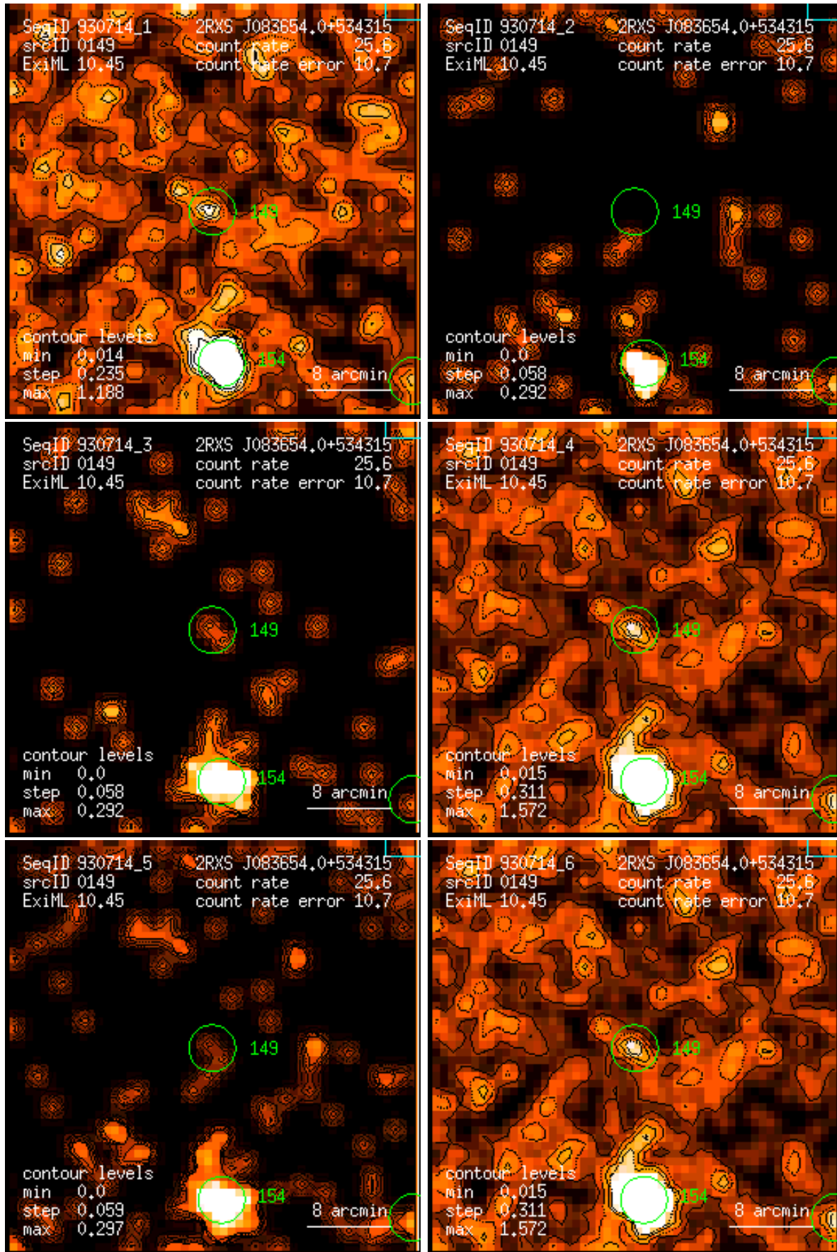
Figure 149: RASS 930714: detection 0149: band rate images, Gaussian filter: (1) PSPC channels 11 – 41, (2) 52 – 90, (3) 91 – 201, (4) 11 – 235, (5) 52 – 201, (6) 11 – 201. Broad band rates in counts/ks. Band rate contour levels in counts/ks/arcmin 2 .
