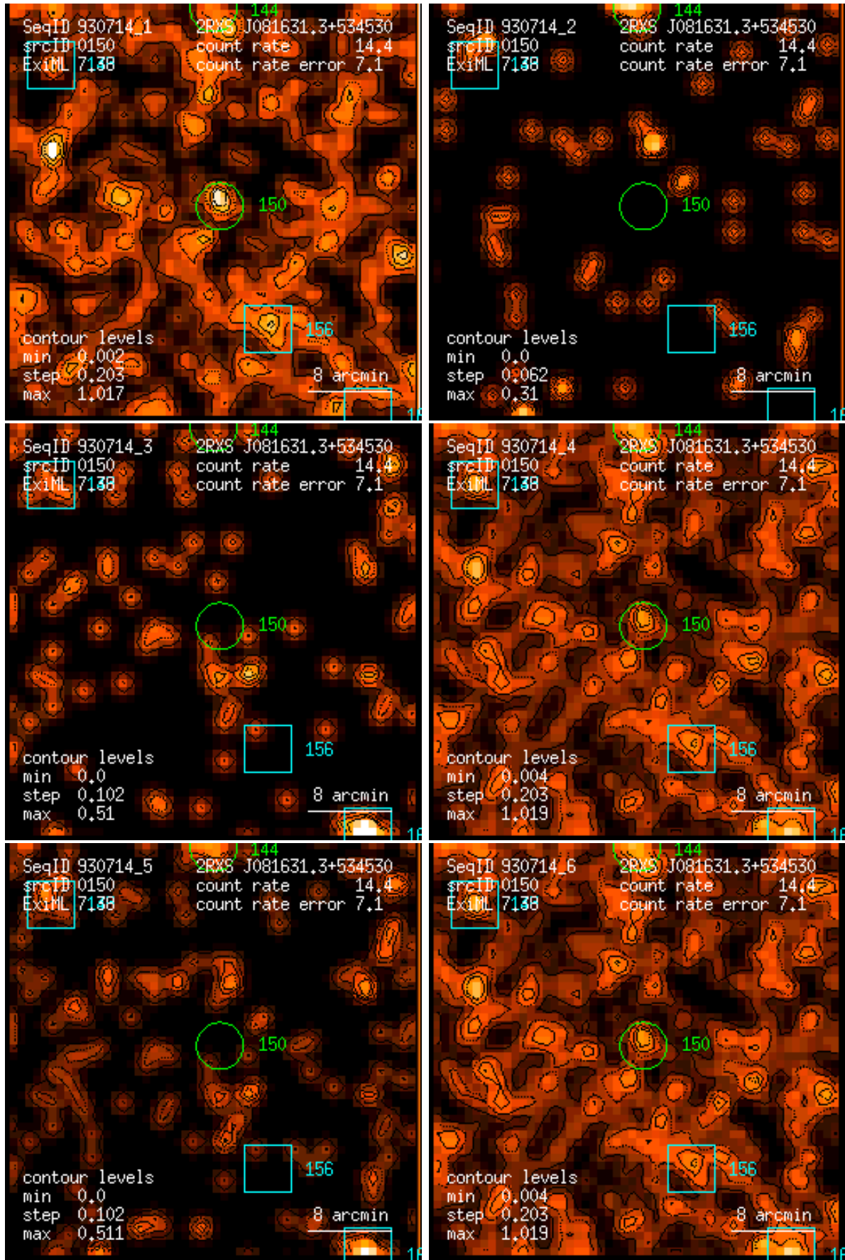
Figure 150: RASS 930714: detection 0150: band rate images, Gaussian filter: (1) PSPC channels 11 – 41, (2) 52 – 90, (3) 91 – 201, (4) 11 – 235, (5) 52 – 201, (6) 11 – 201. Broad band rates in counts/ks. Band rate contour levels in counts/ks/arcmin 2 .
