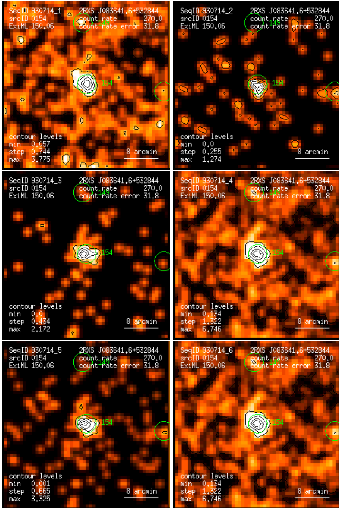
Figure 154: RASS 930714: detection 0154: band rate images, Gaussian filter: (1) PSPC channels 11 – 41, (2) 52 – 90, (3) 91 – 201, (4) 11 – 235, (5) 52 – 201, (6) 11 – 201. Broad band rates in counts/ks. Band rate contour levels in counts/ks/arcmin 2 .
