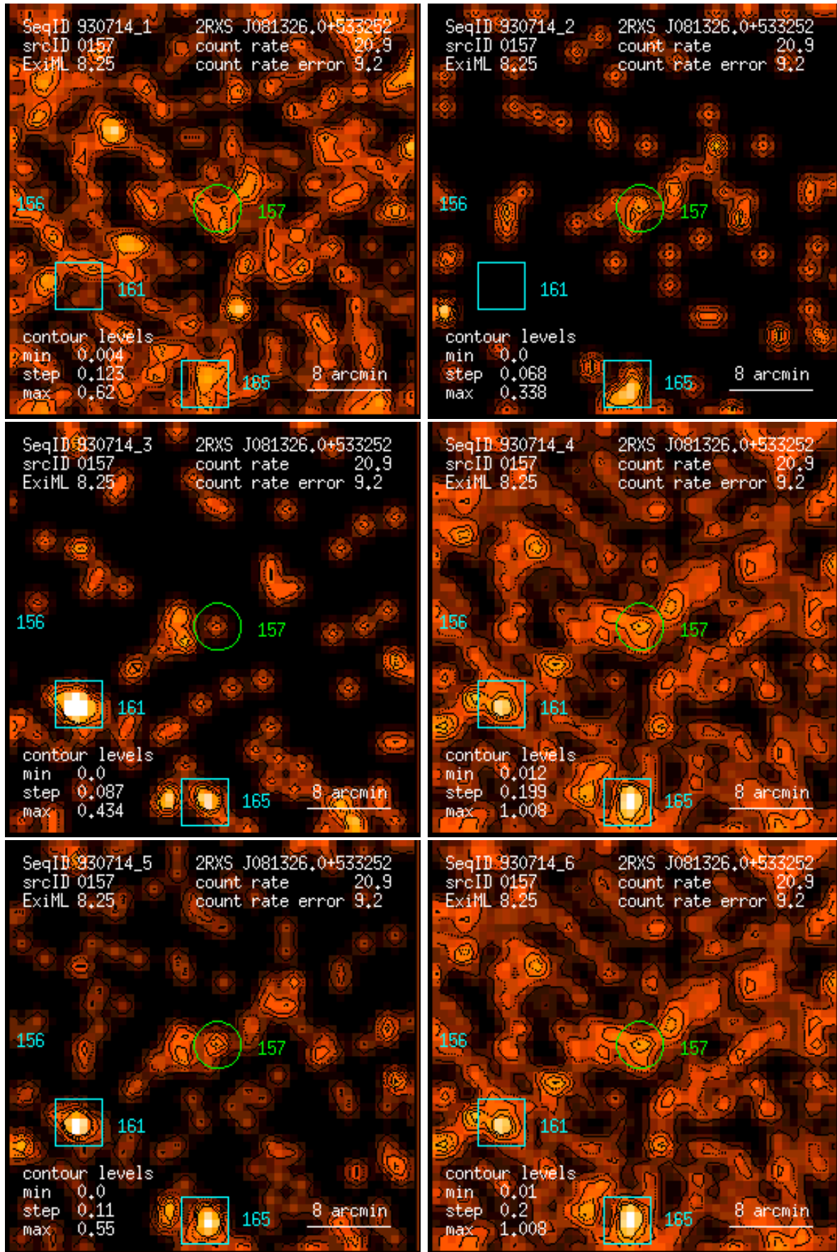
Figure 157: RASS 930714: detection 0157: band rate images, Gaussian filter: (1) PSPC channels 11 – 41, (2) 52 – 90, (3) 91 – 201, (4) 11 – 235, (5) 52 – 201, (6) 11 – 201. Broad band rates in counts/ks. Band rate contour levels in counts/ks/arcmin 2 .
