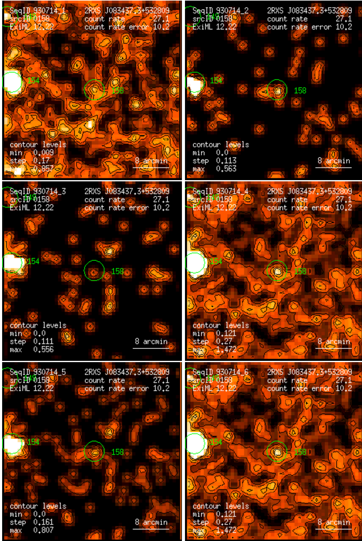
Figure 158: RASS 930714: detection 0158: band rate images, Gaussian filter: (1) PSPC channels 11 – 41, (2) 52 – 90, (3) 91 – 201, (4) 11 – 235, (5) 52 – 201, (6) 11 – 201. Broad band rates in counts/ks. Band rate contour levels in counts/ks/arcmin 2 .
