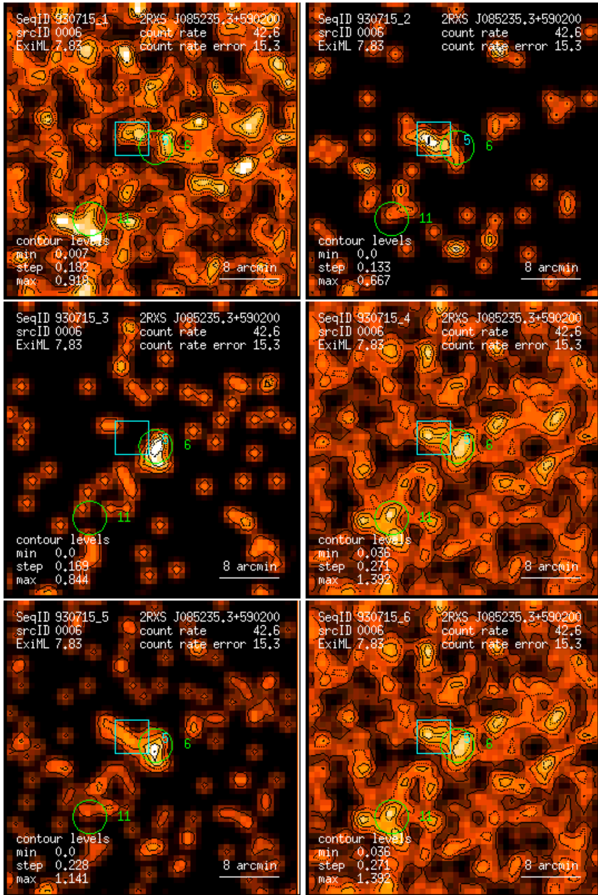
Figure 6: RASS 930715: detection 0006: band rate images, Gaussian filter: (1) PSPC channels 11 – 41, (2) 52 – 90, (3) 91 – 201, (4) 11 – 235, (5) 52 – 201, (6) 11 – 201. Broad band rates in counts/ks. Band rate contour levels in counts/ks/arcmin 2 .
