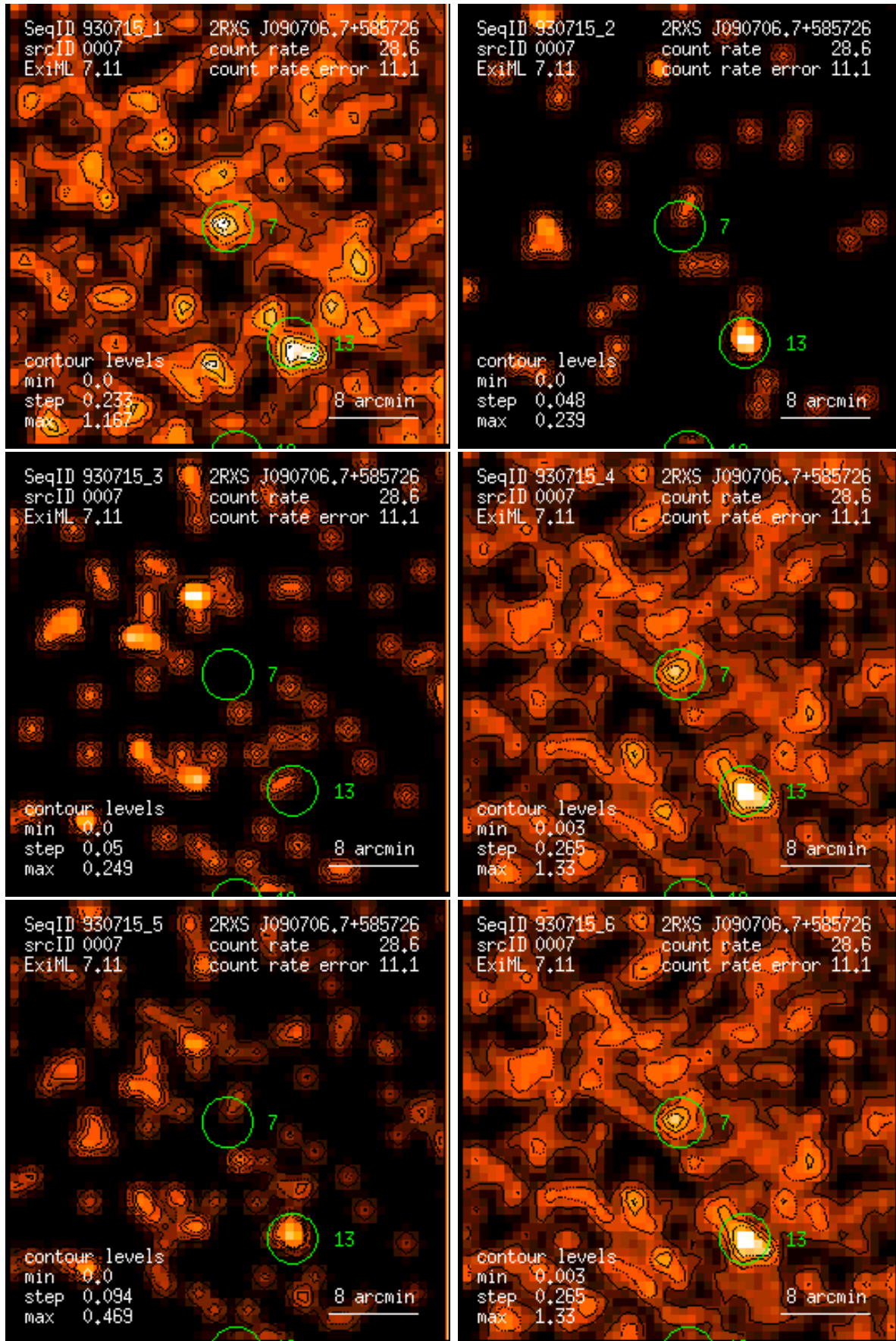
Figure 7: RASS 930715: detection 0007: band rate images, Gaussian filter: (1) PSPC channels 11 – 41, (2) 52 – 90, (3) 91 – 201, (4) 11 – 235, (5) 52 – 201, (6) 11 – 201. Broad band rates in counts/ks. Band rate contour levels in counts/ks/arcmin 2 .
