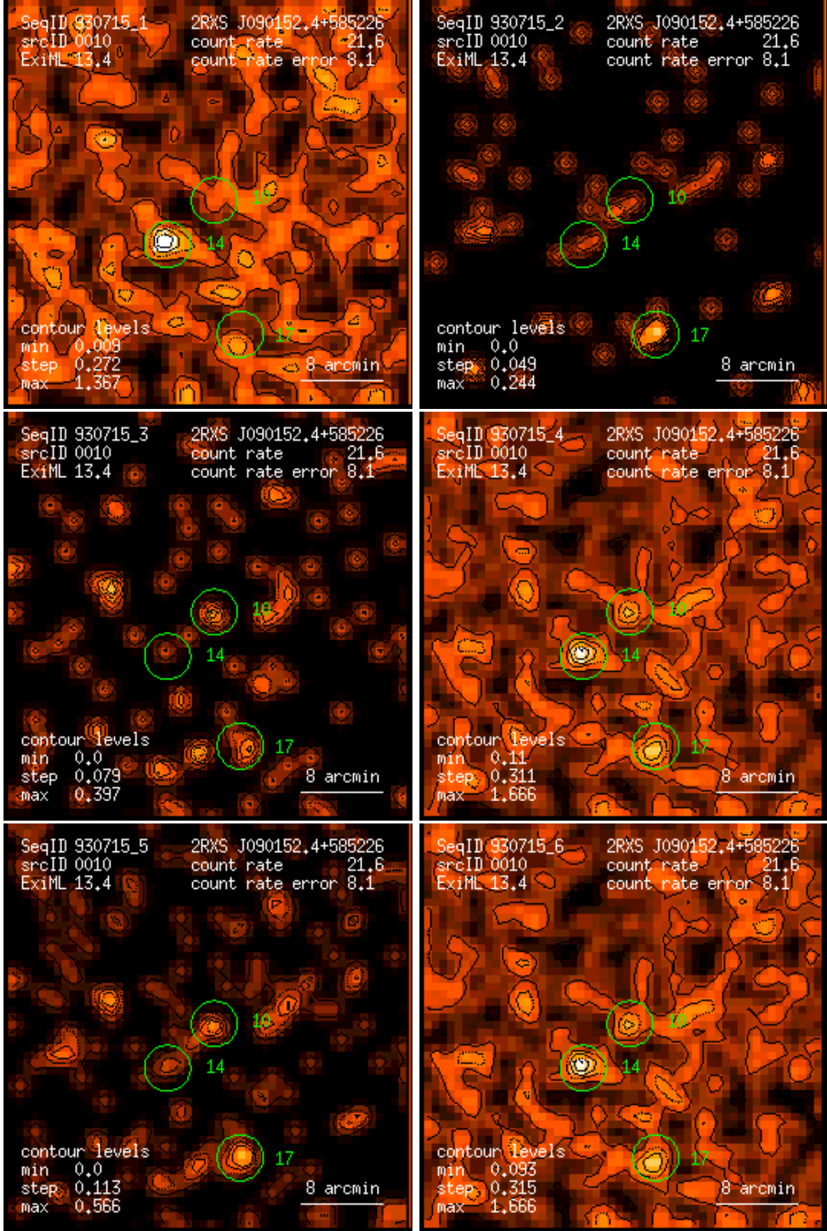
Figure 10: RASS 930715: detection 0010: band rate images, Gaussian filter: (1) PSPC channels 11 – 41, (2) 52 – 90, (3) 91 – 201, (4) 11 – 235, (5) 52 – 201, (6) 11 – 201. Broad band rates in counts/ks. Band rate contour levels in counts/ks/arcmin 2 .
