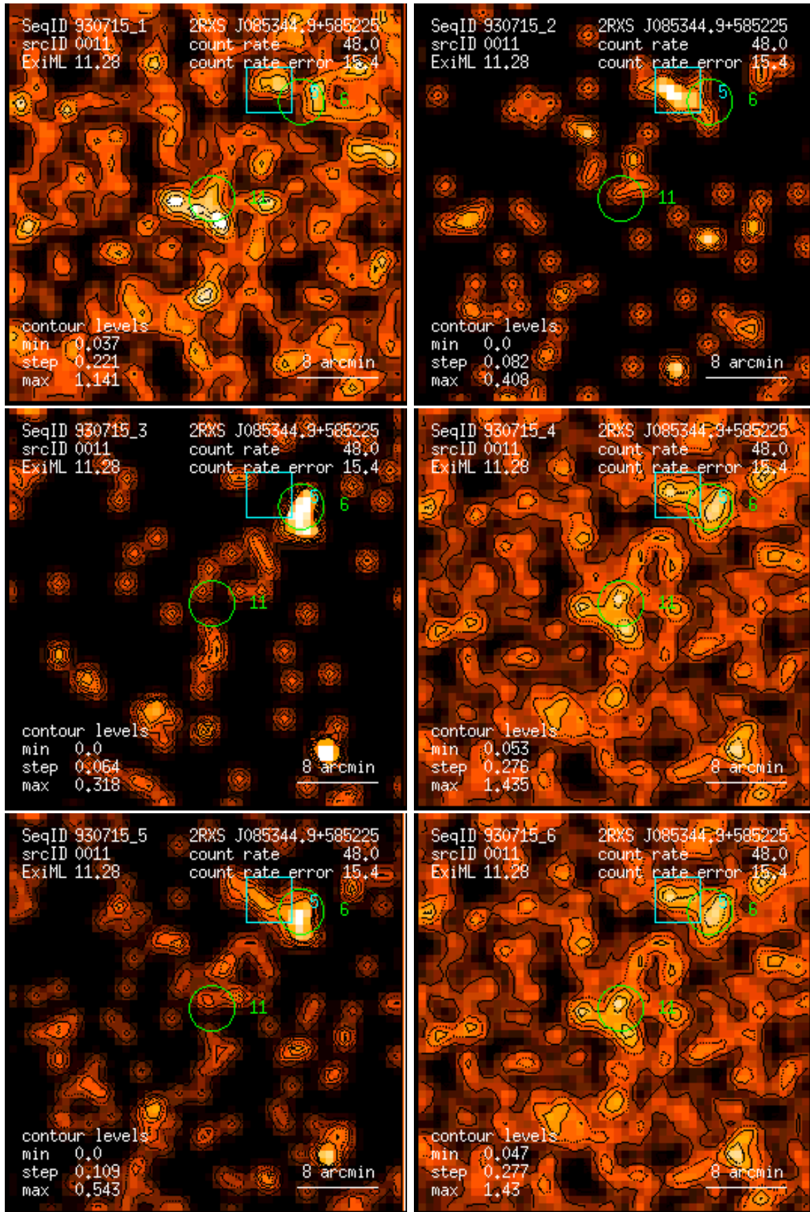
Figure 11: RASS 930715: detection 0011: band rate images, Gaussian filter: (1) PSPC channels 11 – 41, (2) 52 – 90, (3) 91 – 201, (4) 11 – 235, (5) 52 – 201, (6) 11 – 201. Broad band rates in counts/ks. Band rate contour levels in counts/ks/arcmin 2 .
