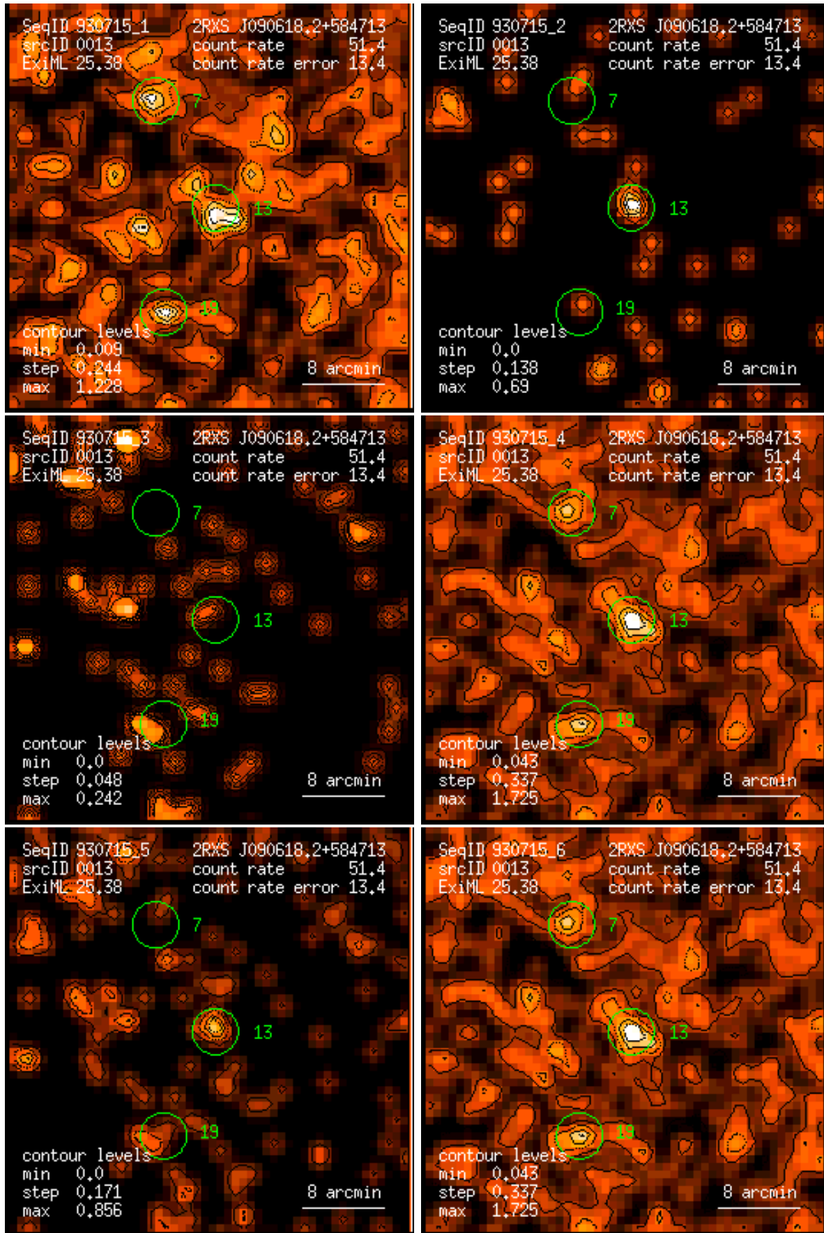
Figure 13: RASS 930715: detection 0013: band rate images, Gaussian filter: (1) PSPC channels 11 – 41, (2) 52 – 90, (3) 91 – 201, (4) 11 – 235, (5) 52 – 201, (6) 11 – 201. Broad band rates in counts/ks. Band rate contour levels in counts/ks/arcmin 2 .
