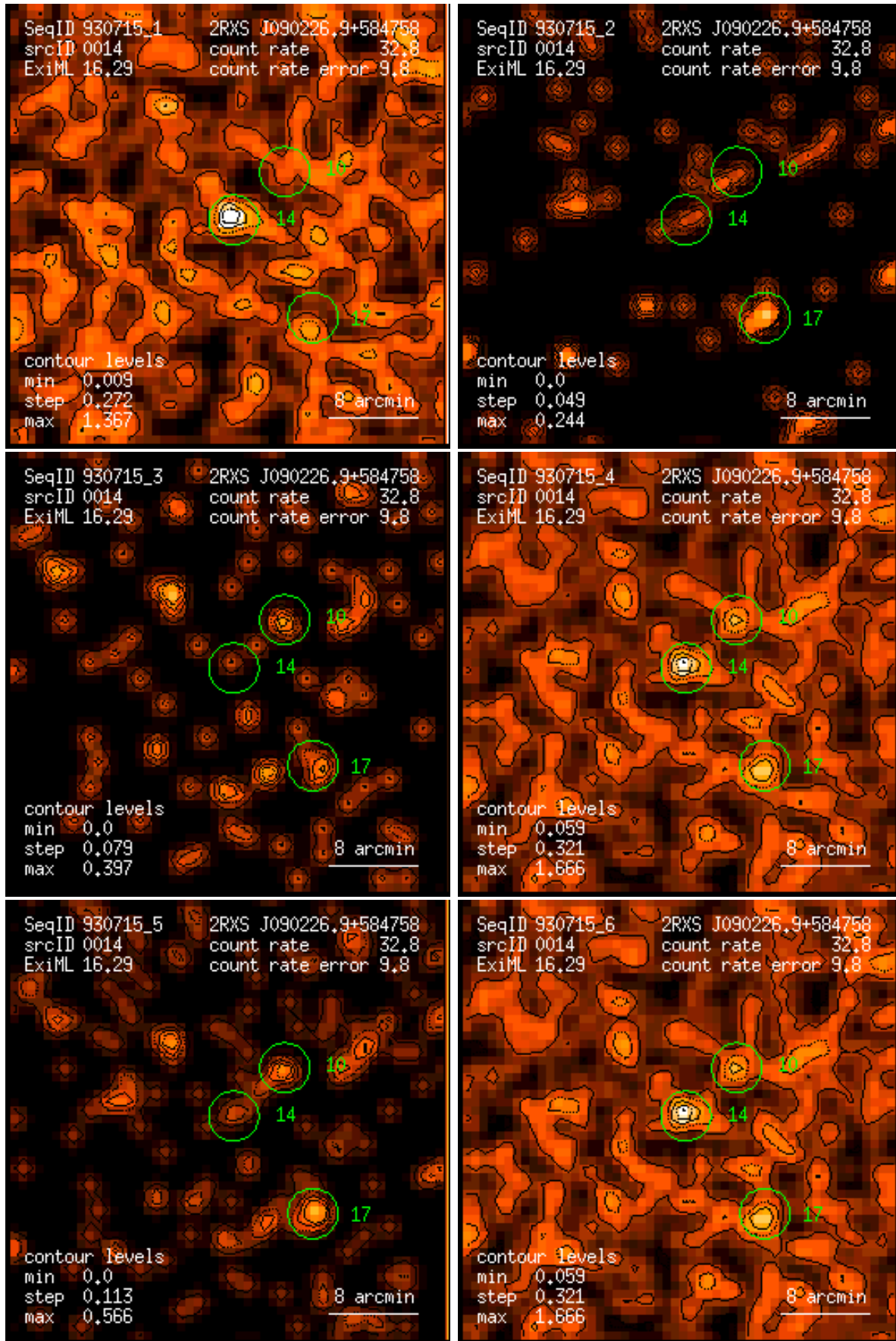
Figure 14: RASS 930715: detection 0014: band rate images, Gaussian filter: (1) PSPC channels 11 – 41, (2) 52 – 90, (3) 91 – 201, (4) 11 – 235, (5) 52 – 201, (6) 11 – 201. Broad band rates in counts/ks. Band rate contour levels in counts/ks/arcmin 2 .
