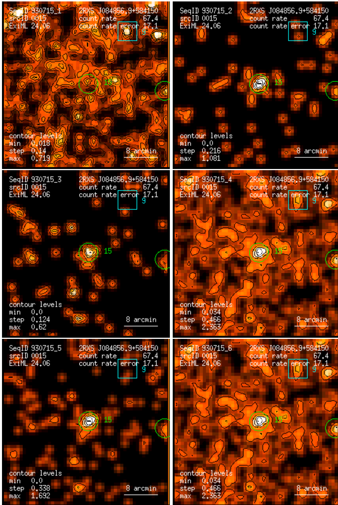
Figure 15: RASS 930715: detection 0015: band rate images, Gaussian filter: (1) PSPC channels 11 – 41, (2) 52 – 90, (3) 91 – 201, (4) 11 – 235, (5) 52 – 201, (6) 11 – 201. Broad band rates in counts/ks. Band rate contour levels in counts/ks/arcmin 2 .
