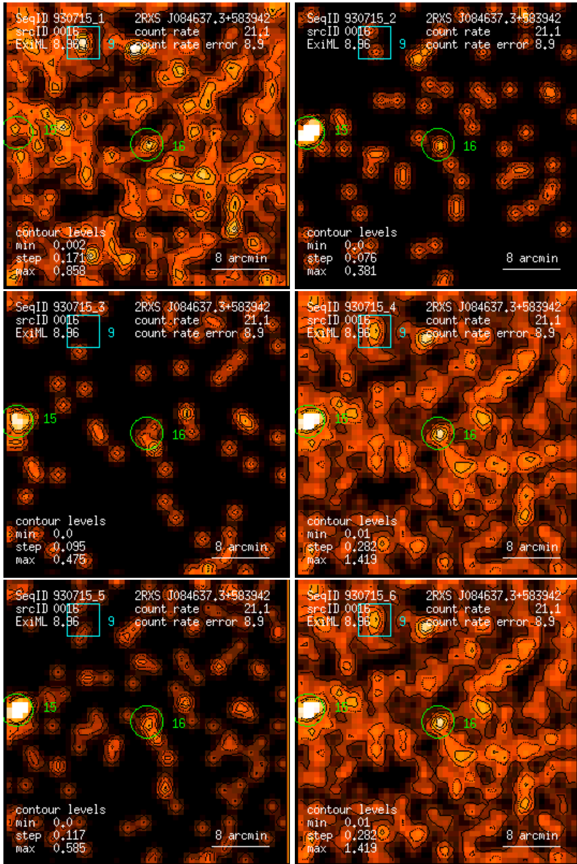
Figure 16: RASS 930715: detection 0016: band rate images, Gaussian filter: (1) PSPC channels 11 – 41, (2) 52 – 90, (3) 91 – 201, (4) 11 – 235, (5) 52 – 201, (6) 11 – 201. Broad band rates in counts/ks. Band rate contour levels in counts/ks/arcmin 2 .
