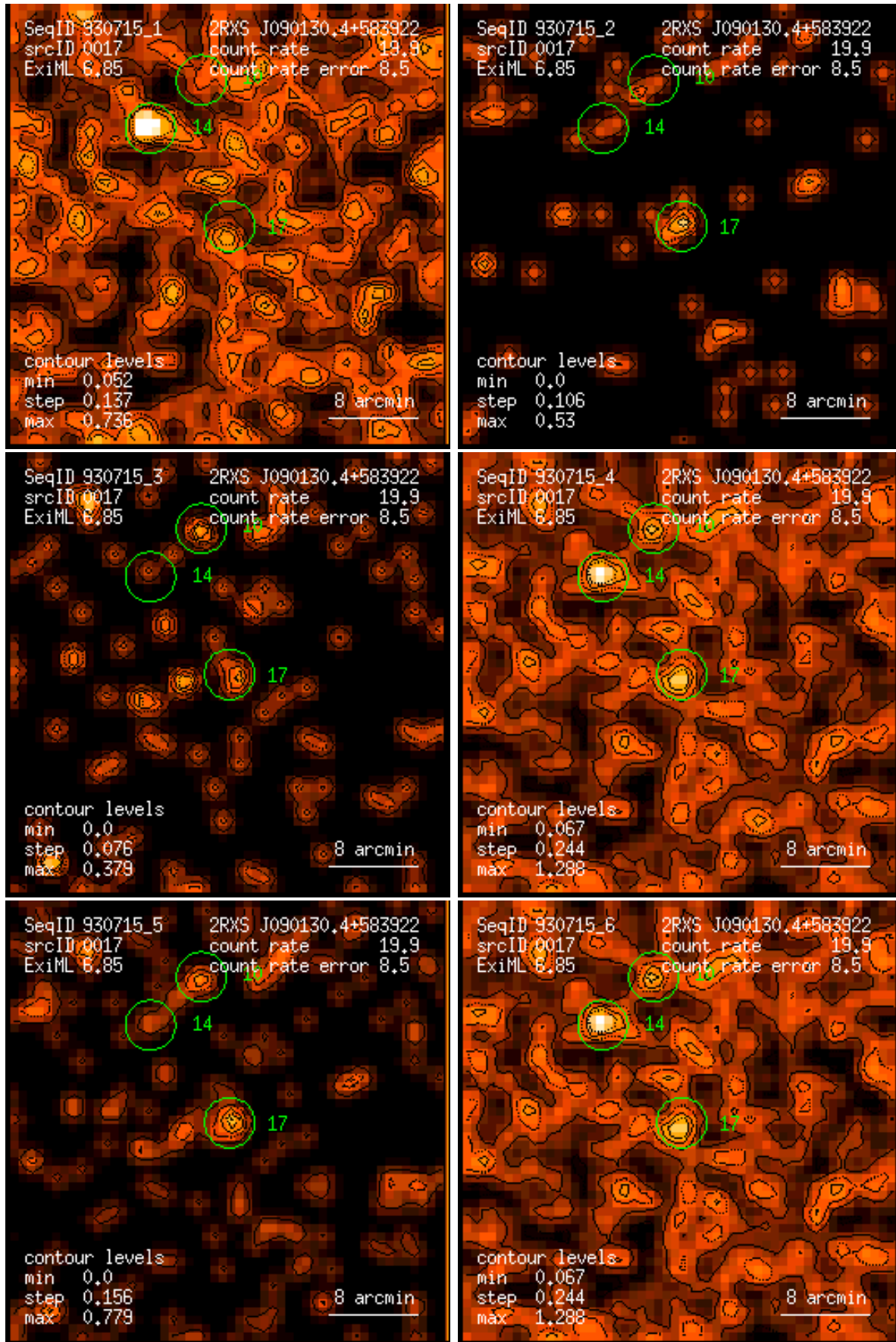
Figure 17: RASS 930715: detection 0017: band rate images, Gaussian filter: (1) PSPC channels 11 – 41, (2) 52 – 90, (3) 91 – 201, (4) 11 – 235, (5) 52 – 201, (6) 11 – 201. Broad band rates in counts/ks. Band rate contour levels in counts/ks/arcmin 2 .
