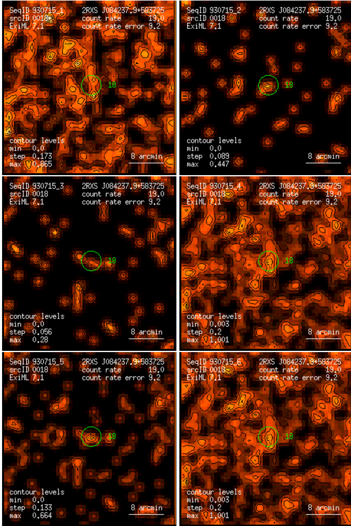
Figure 18: RASS 930715: detection 0018: band rate images, Gaussian filter: (1) PSPC channels 11 – 41, (2) 52 – 90, (3) 91 – 201, (4) 11 – 235, (5) 52 – 201, (6) 11 – 201. Broad band rates in counts/ks. Band rate contour levels in counts/ks/arcmin 2 .
