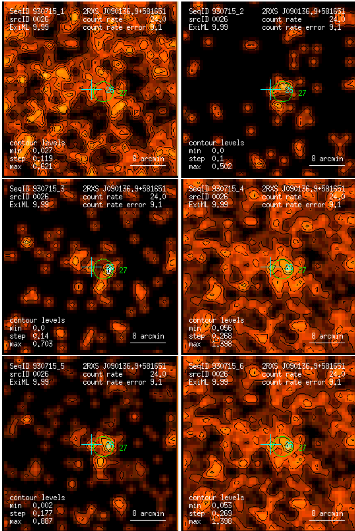
Figure 26: RASS 930715: detection 0026: band rate images, Gaussian filter: (1) PSPC channels 11 – 41, (2) 52 – 90, (3) 91 – 201, (4) 11 – 235, (5) 52 – 201, (6) 11 – 201. Broad band rates in counts/ks. Band rate contour levels in counts/ks/arcmin 2 .
