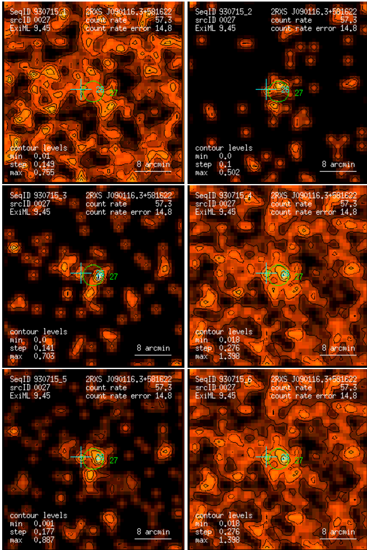
Figure 27: RASS 930715: detection 0027: band rate images, Gaussian filter: (1) PSPC channels 11 – 41, (2) 52 – 90, (3) 91 – 201, (4) 11 – 235, (5) 52 – 201, (6) 11 – 201. Broad band rates in counts/ks. Band rate contour levels in counts/ks/arcmin 2 .
