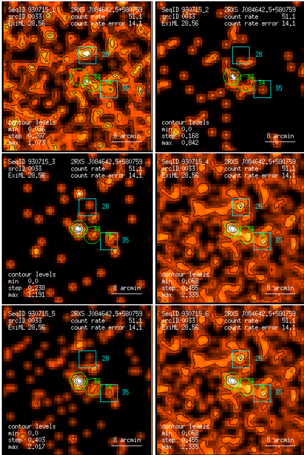
Figure 33: RASS 930715: detection 0033: band rate images, Gaussian filter: (1) PSPC channels 11 – 41, (2) 52 – 90, (3) 91 – 201, (4) 11 – 235, (5) 52 – 201, (6) 11 – 201. Broad band rates in counts/ks. Band rate contour levels in counts/ks/arcmin 2 .
