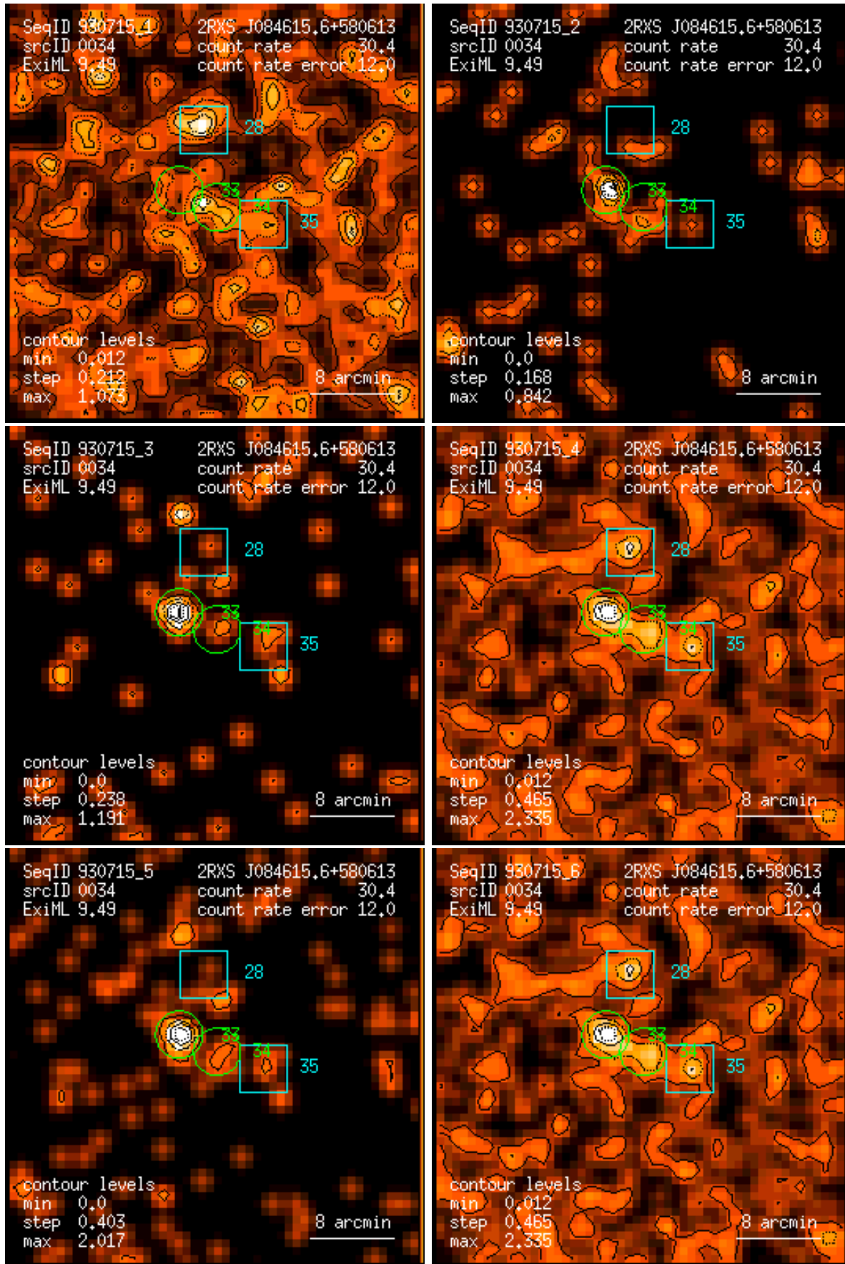
Figure 34: RASS 930715: detection 0034: band rate images, Gaussian filter: (1) PSPC channels 11 – 41, (2) 52 – 90, (3) 91 – 201, (4) 11 – 235, (5) 52 – 201, (6) 11 – 201. Broad band rates in counts/ks. Band rate contour levels in counts/ks/arcmin 2 .
