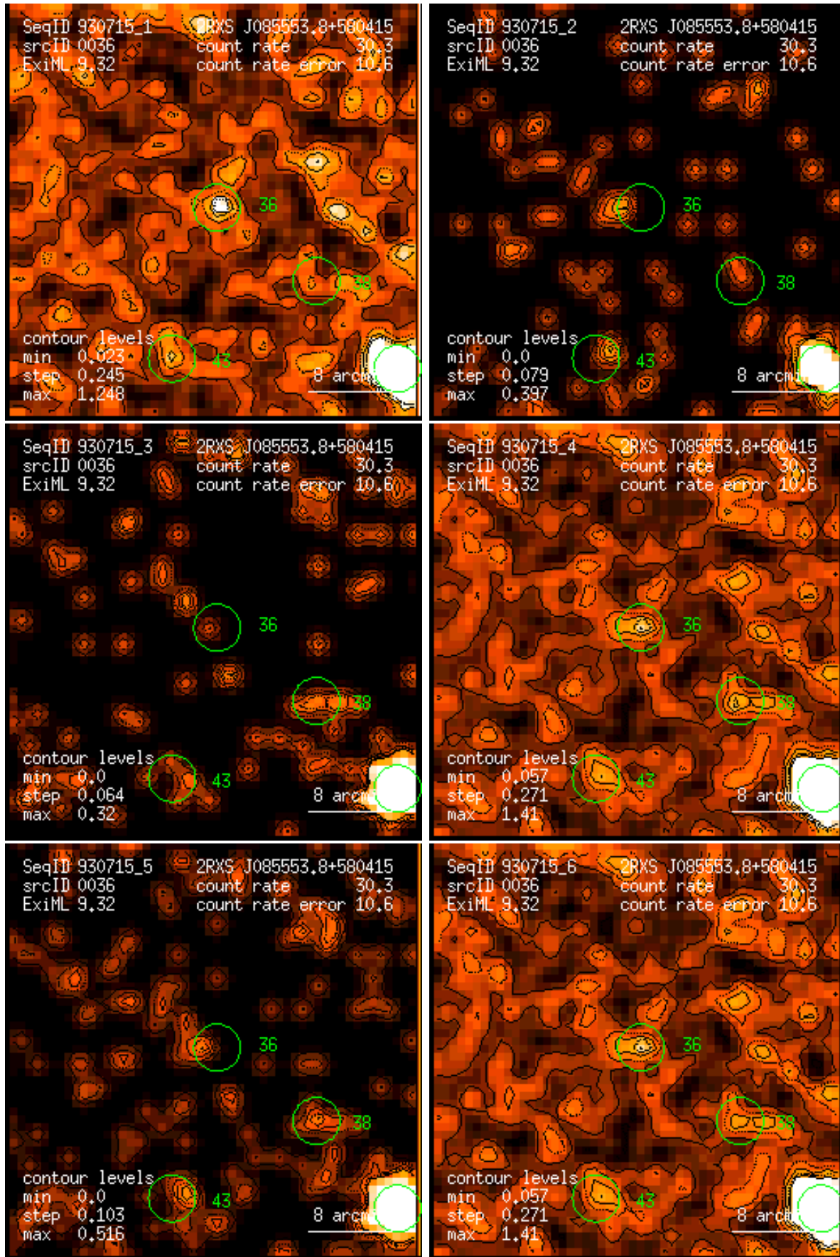
Figure 36: RASS 930715: detection 0036: band rate images, Gaussian filter: (1) PSPC channels 11 – 41, (2) 52 – 90, (3) 91 – 201, (4) 11 – 235, (5) 52 – 201, (6) 11 – 201. Broad band rates in counts/ks. Band rate contour levels in counts/ks/arcmin 2 .
