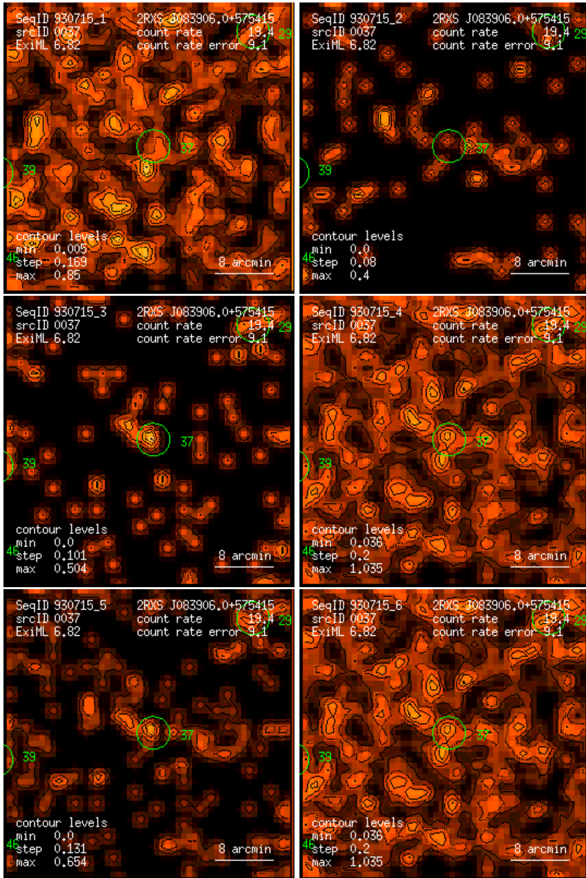
Figure 37: RASS 930715: detection 0037: band rate images, Gaussian filter: (1) PSPC channels 11 – 41, (2) 52 – 90, (3) 91 – 201, (4) 11 – 235, (5) 52 – 201, (6) 11 – 201. Broad band rates in counts/ks. Band rate contour levels in counts/ks/arcmin 2 .
