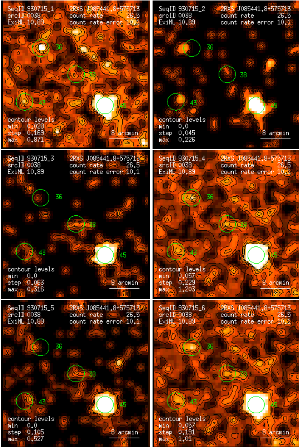
Figure 38: RASS 930715: detection 0038: band rate images, Gaussian filter: (1) PSPC channels 11 – 41, (2) 52 – 90, (3) 91 – 201, (4) 11 – 235, (5) 52 – 201, (6) 11 – 201. Broad band rates in counts/ks. Band rate contour levels in counts/ks/arcmin 2 .
