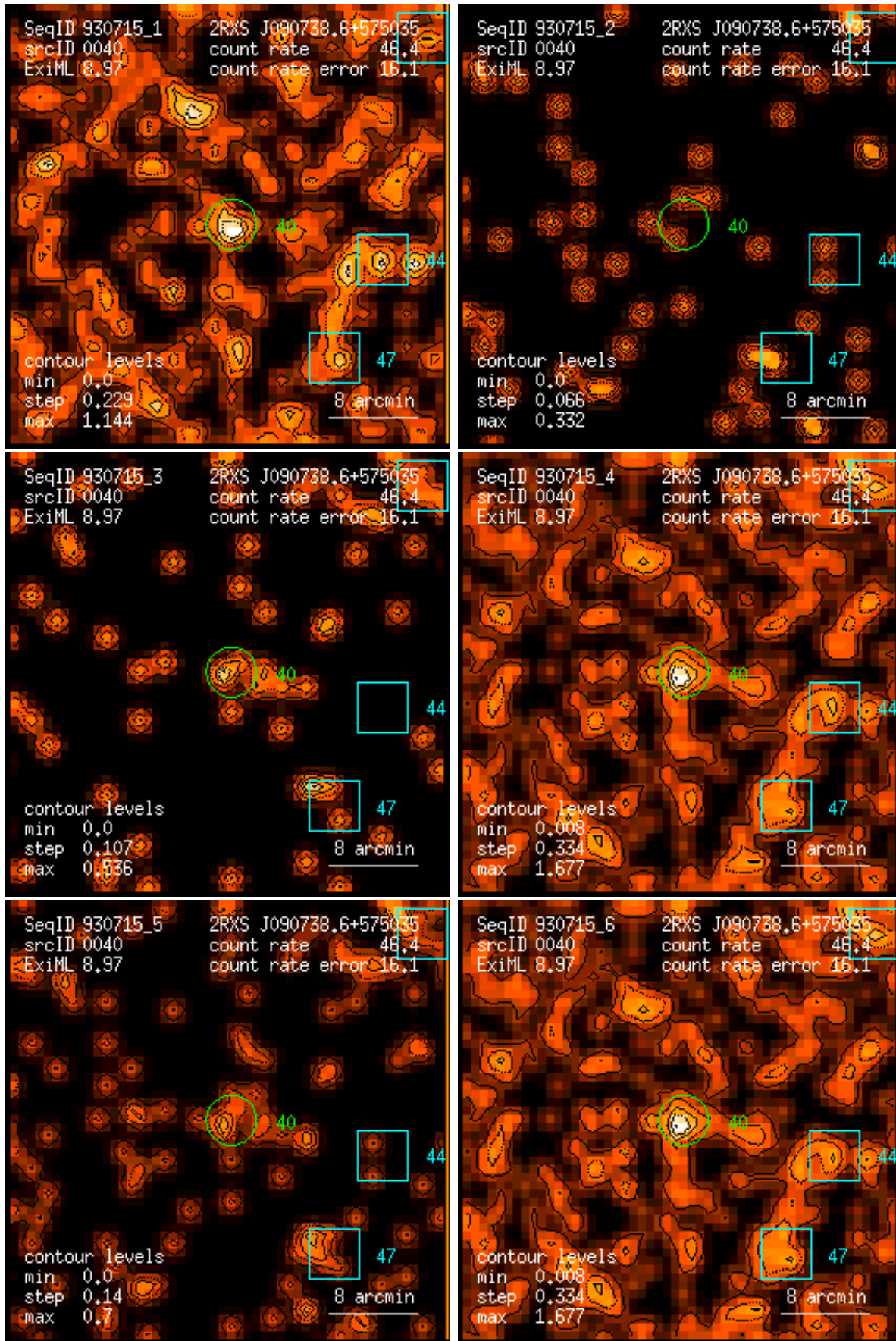
Figure 40: RASS 930715: detection 0040: band rate images, Gaussian filter: (1) PSPC channels 11 – 41, (2) 52 – 90, (3) 91 – 201, (4) 11 – 235, (5) 52 – 201, (6) 11 – 201. Broad band rates in counts/ks. Band rate contour levels in counts/ks/arcmin 2 .
