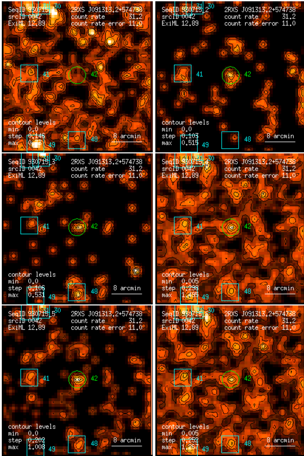
Figure 42: RASS 930715: detection 0042: band rate images, Gaussian filter: (1) PSPC channels 11 – 41, (2) 52 – 90, (3) 91 – 201, (4) 11 – 235, (5) 52 – 201, (6) 11 – 201. Broad band rates in counts/ks. Band rate contour levels in counts/ks/arcmin 2 .
