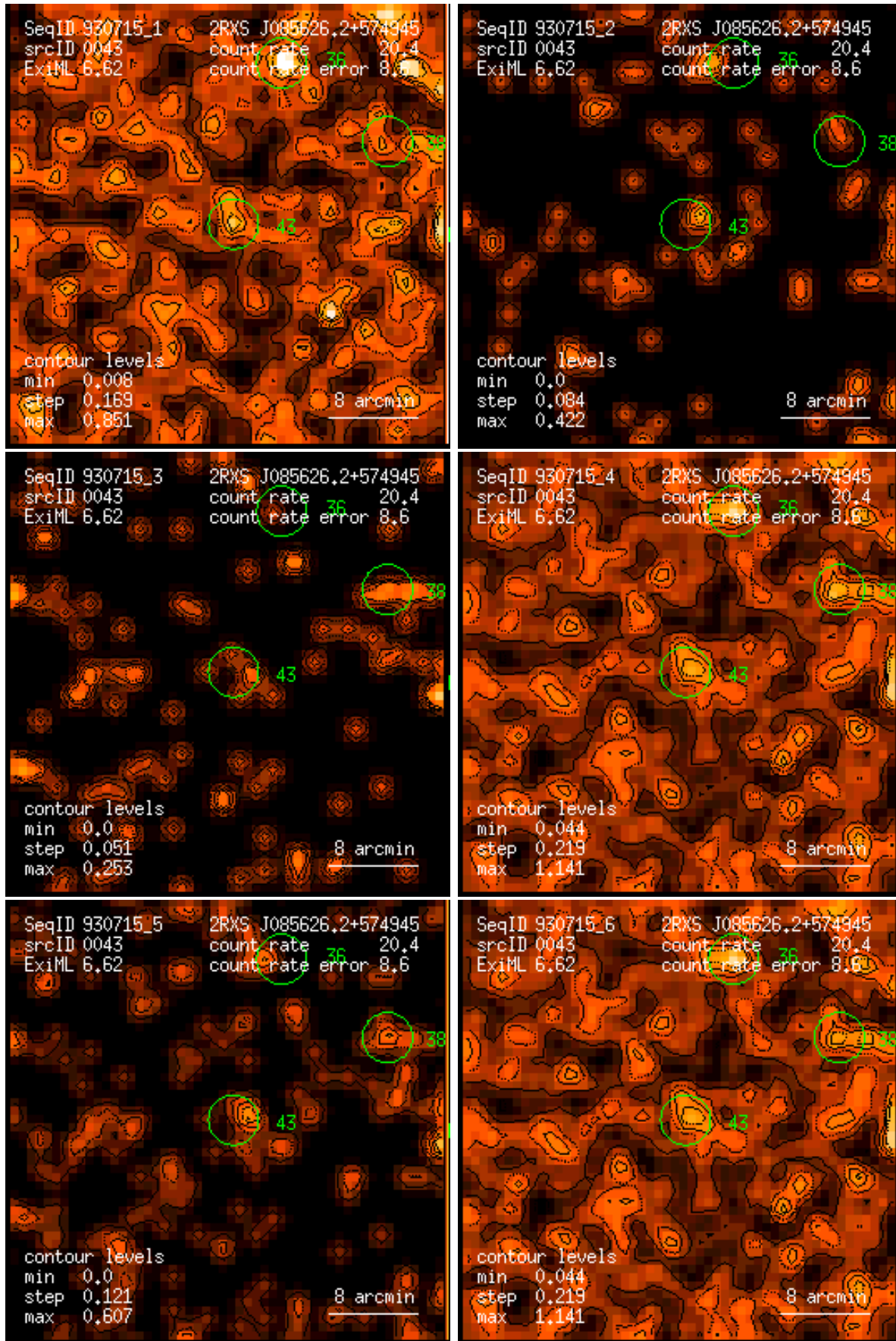
Figure 43: RASS 930715: detection 0043: band rate images, Gaussian filter: (1) PSPC channels 11 – 41, (2) 52 – 90, (3) 91 – 201, (4) 11 – 235, (5) 52 – 201, (6) 11 – 201. Broad band rates in counts/ks. Band rate contour levels in counts/ks/arcmin 2 .
