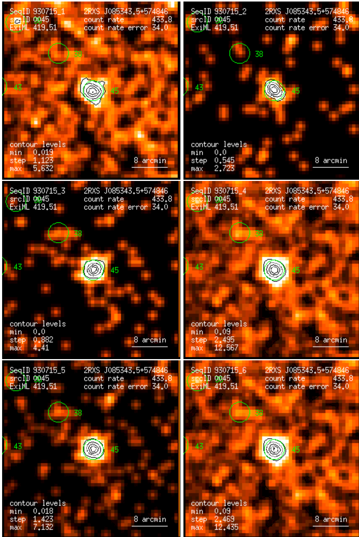
Figure 45: RASS 930715: detection 0045: band rate images, Gaussian filter: (1) PSPC channels 11 – 41, (2) 52 – 90, (3) 91 – 201, (4) 11 – 235, (5) 52 – 201, (6) 11 – 201. Broad band rates in counts/ks. Band rate contour levels in counts/ks/arcmin 2 .
