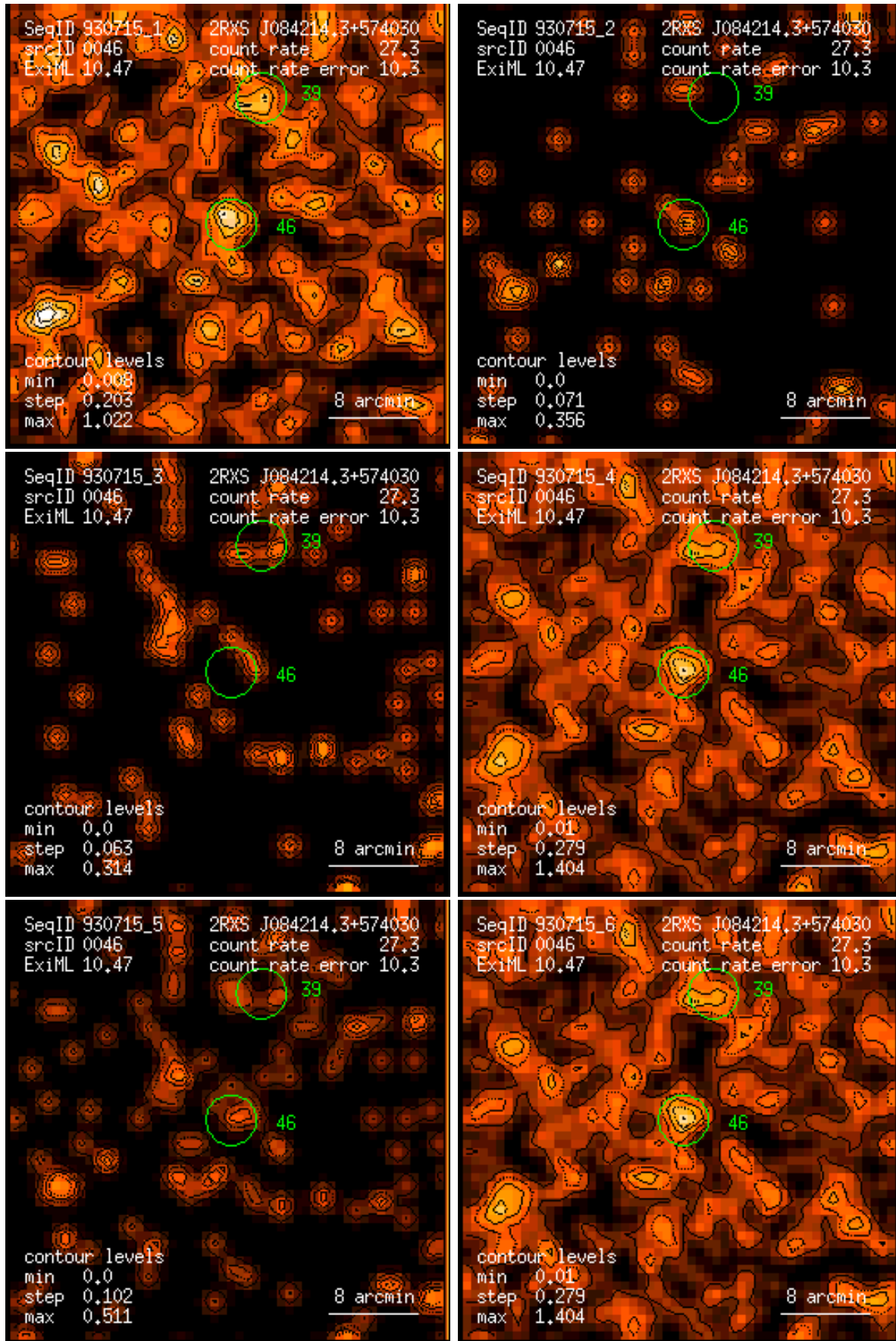
Figure 46: RASS 930715: detection 0046: band rate images, Gaussian filter: (1) PSPC channels 11 – 41, (2) 52 – 90, (3) 91 – 201, (4) 11 – 235, (5) 52 – 201, (6) 11 – 201. Broad band rates in counts/ks. Band rate contour levels in counts/ks/arcmin 2 .
